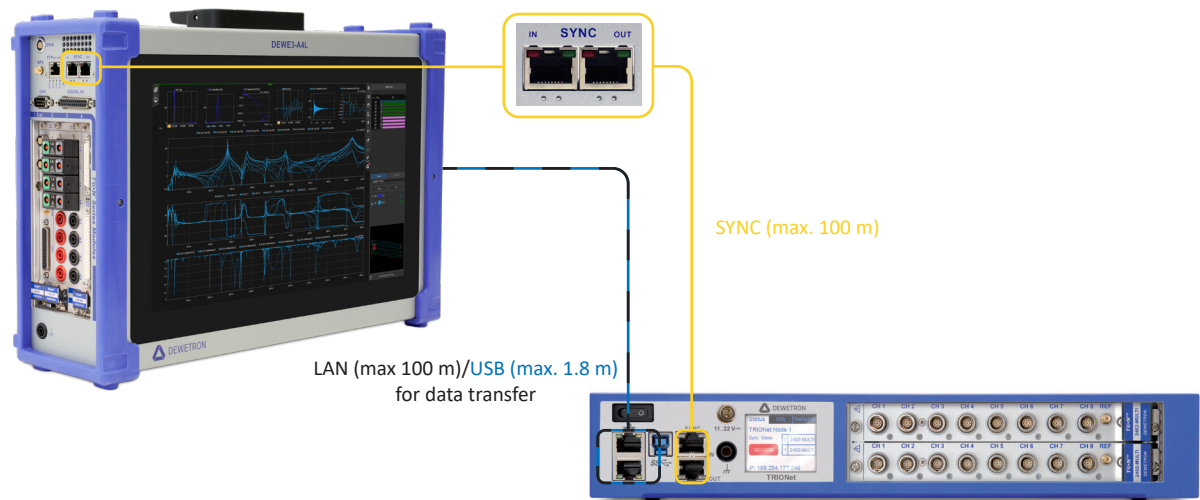
Fig. 28: Channel expansion with TRIONet
