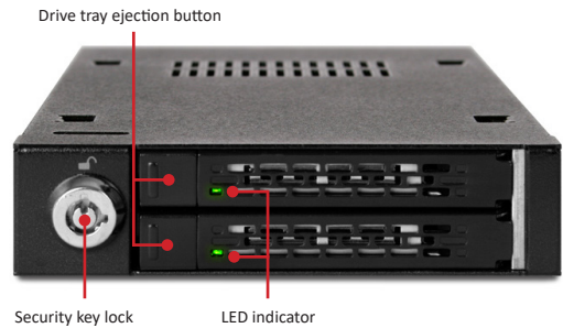
Fig. 17: Dual SSD drive bay
