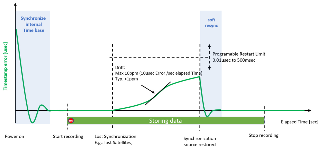
Fig. 5: Gapless recording
