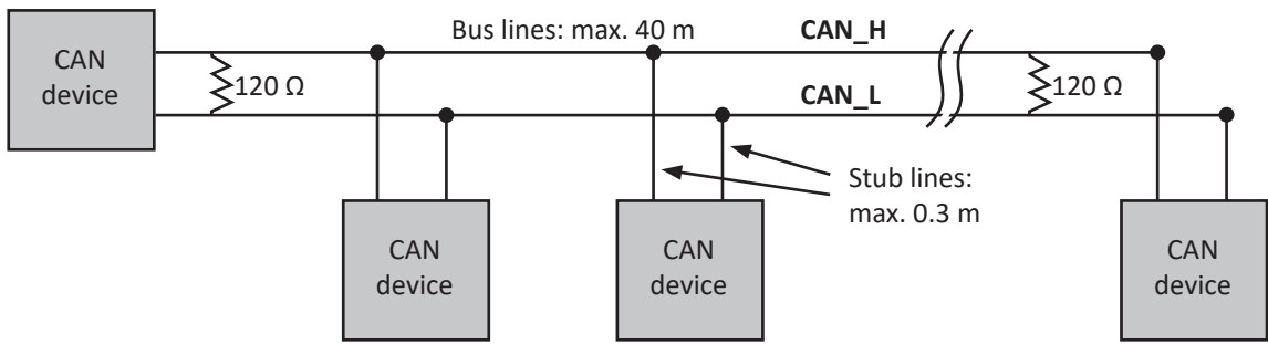
Fig. 11: High-speed CAN
