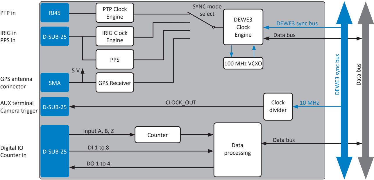
Fig. 4: Signal routing
