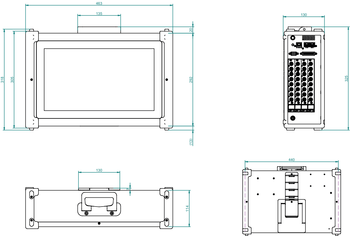
Fig. 1: Dimensions DEWE3-A4L
