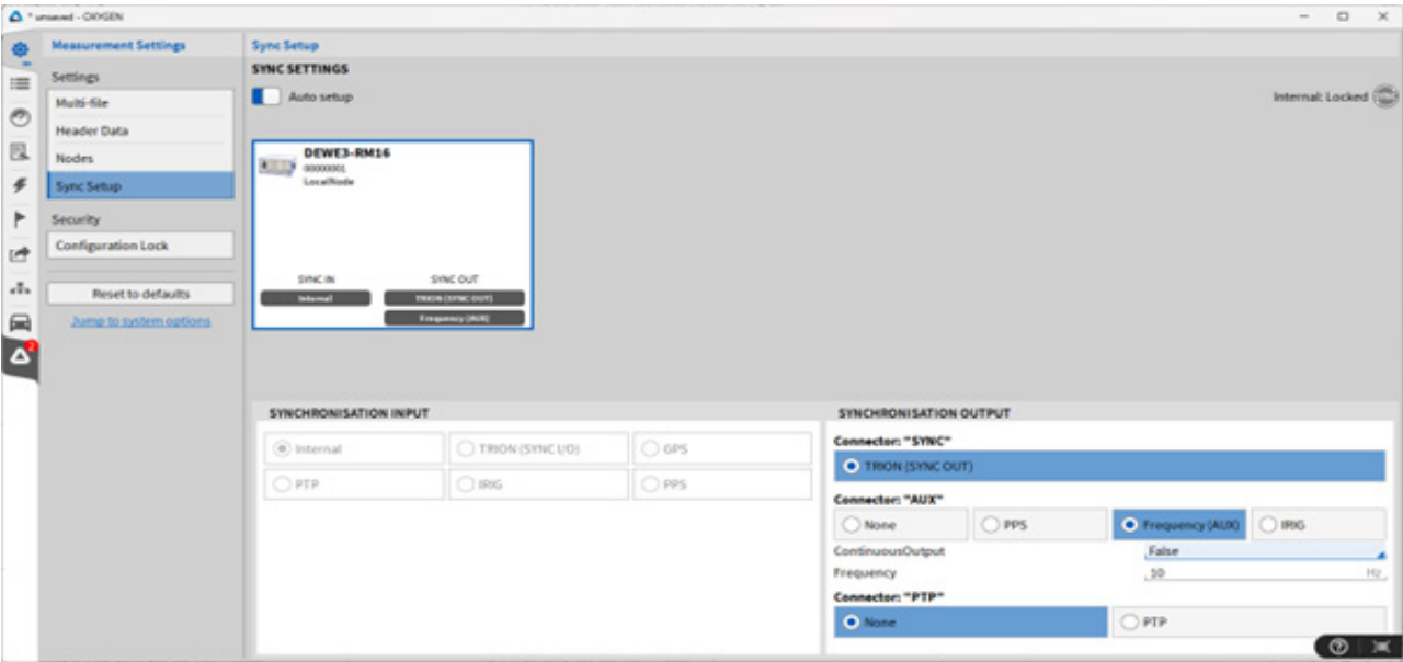
Fig. 8: Output settings
