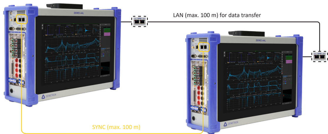
Fig. 29: Network with multiple systems
