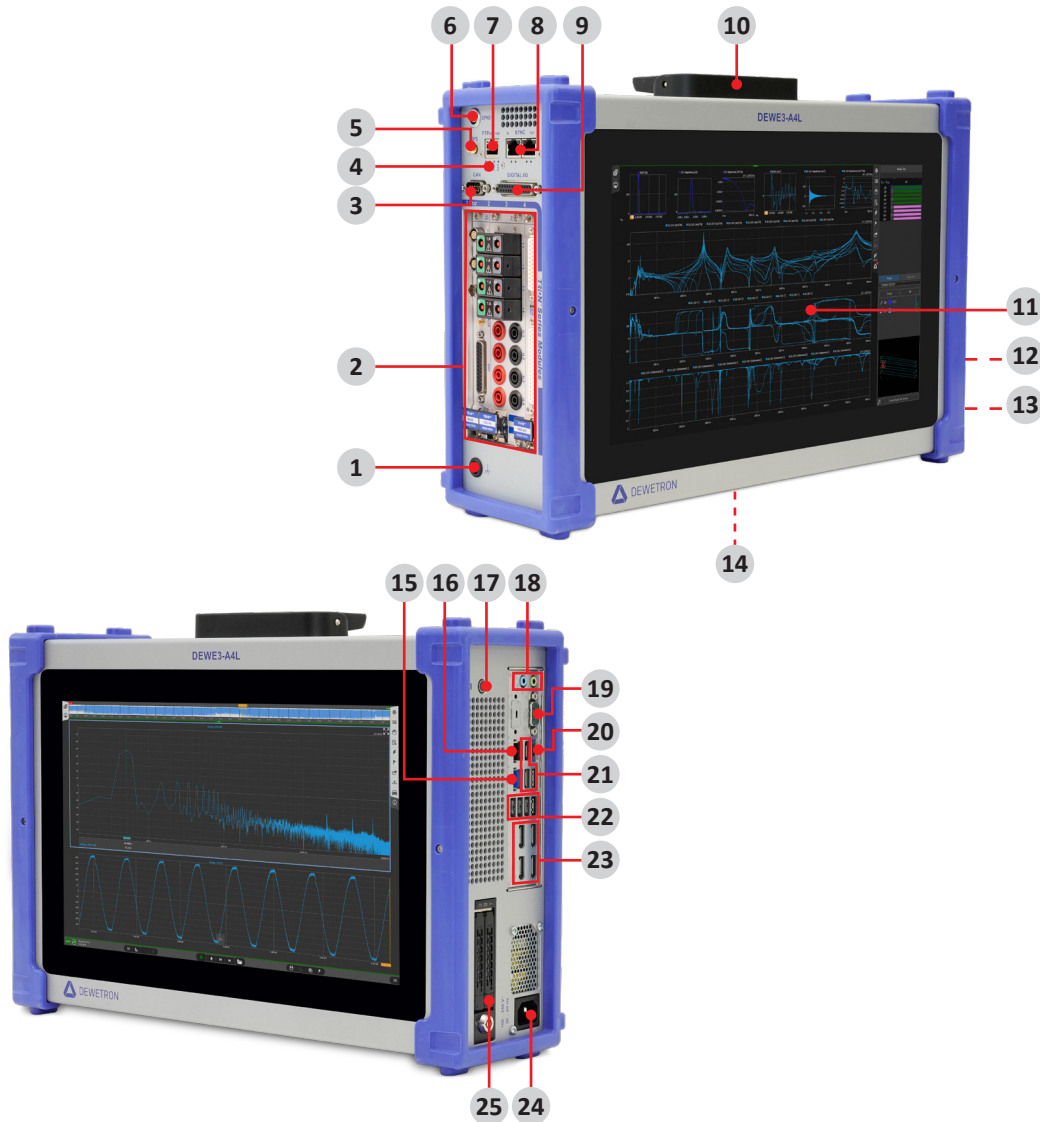
Fig. 3: DEWE3-A4L connections and ports
