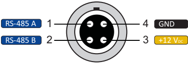
Fig. 13: Pin assignment EPAD2 connector
