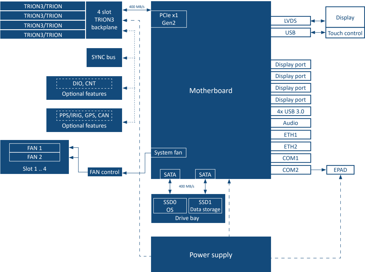
Fig. 2: Block diagram
