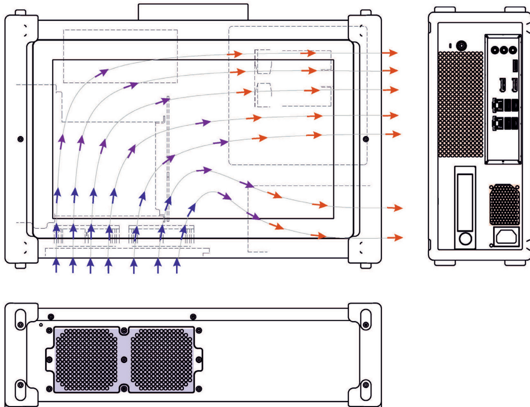
Fig. 19: Cooling concept
