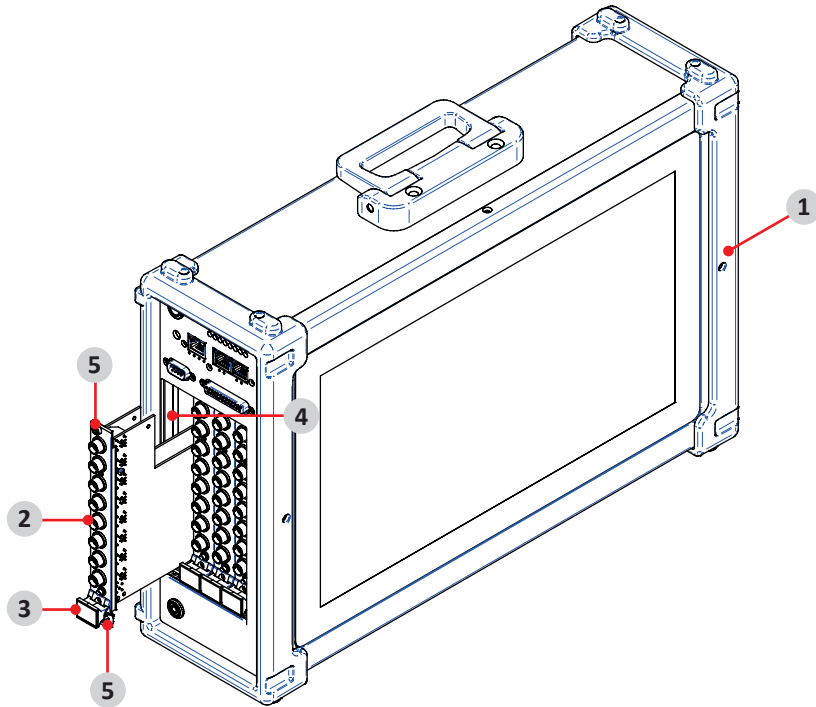
Fig. 18: Installing a TRION module
