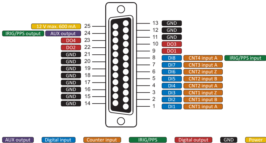
Fig. 7: Pin assignment D-SUB-25 connector
