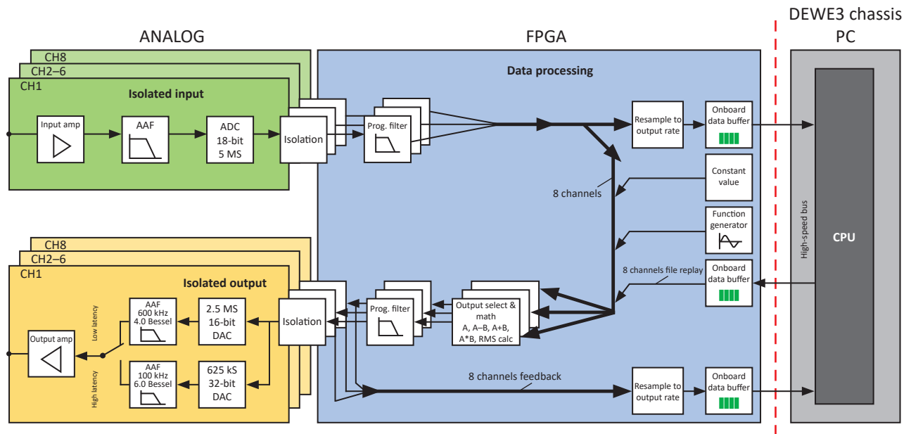
Fig. 25: Simplified signal path
