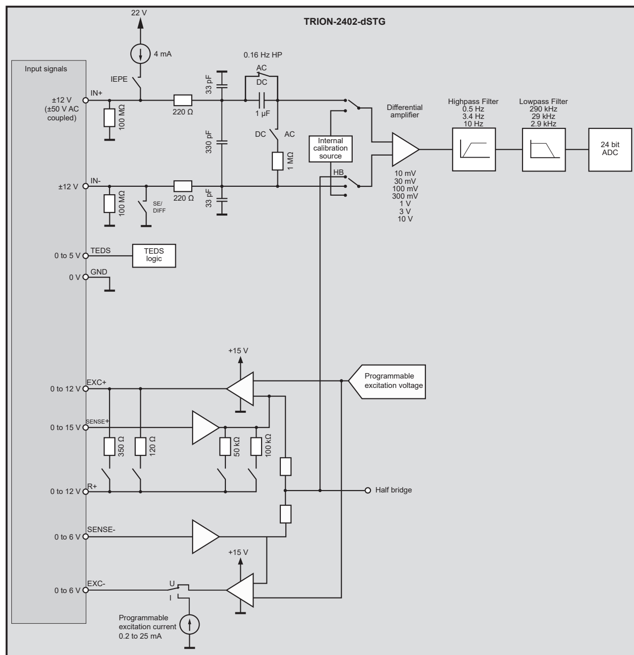
Fig. 132: Block diagram
