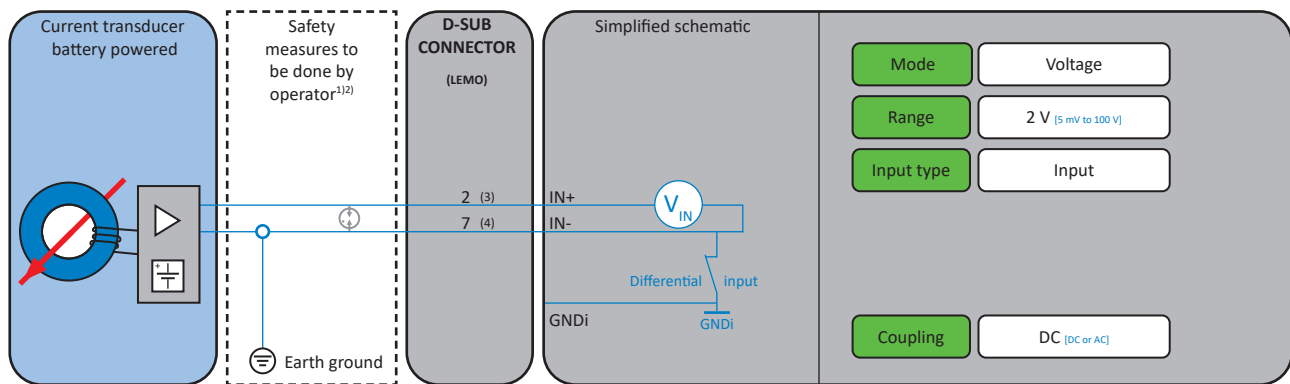
Fig. 31: Current transducer with voltage output
