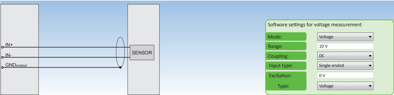
Fig. 118: Voltage measurement
