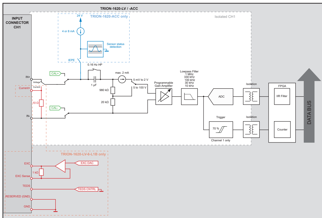
Fig. 92: Base block diagram of the TRION-1620-ACC/LV module
