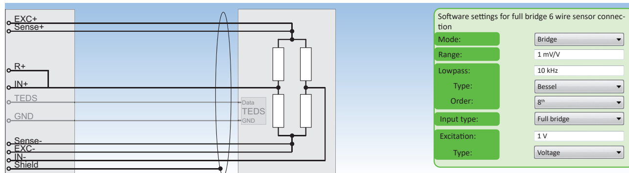
Fig. 61: Full bridge 6-wire sensor connection
