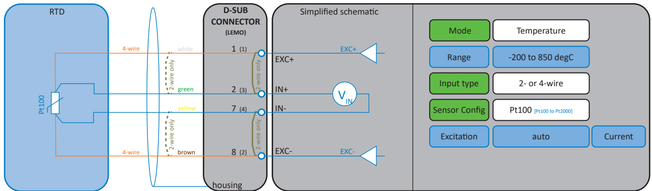
Fig. 47: RTD 2- and 4-wire temperature measurement
