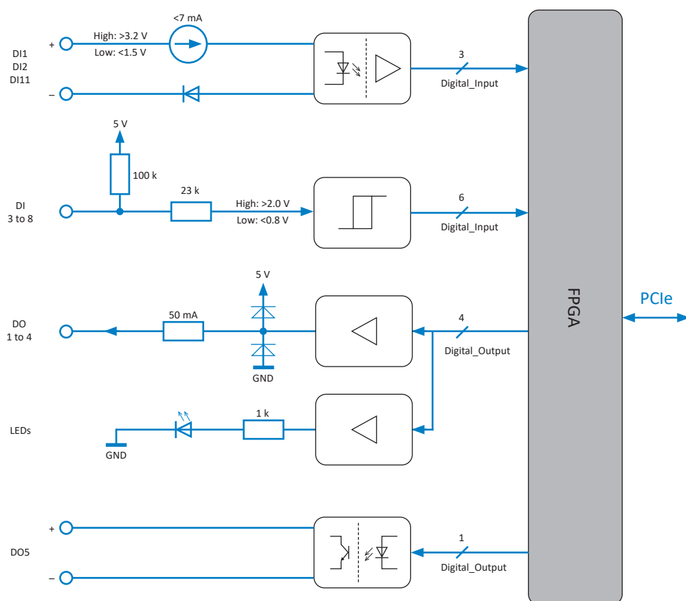
Fig. 178: Digital block diagram
