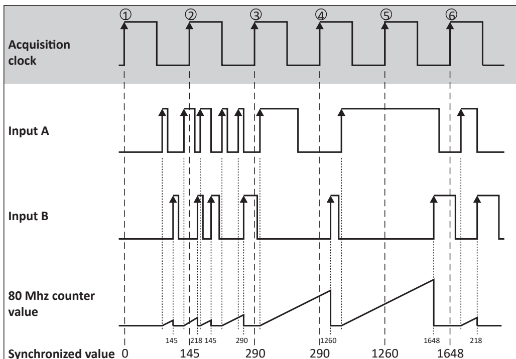
Fig. 210: Two Pulse Edge Separation Measurement
