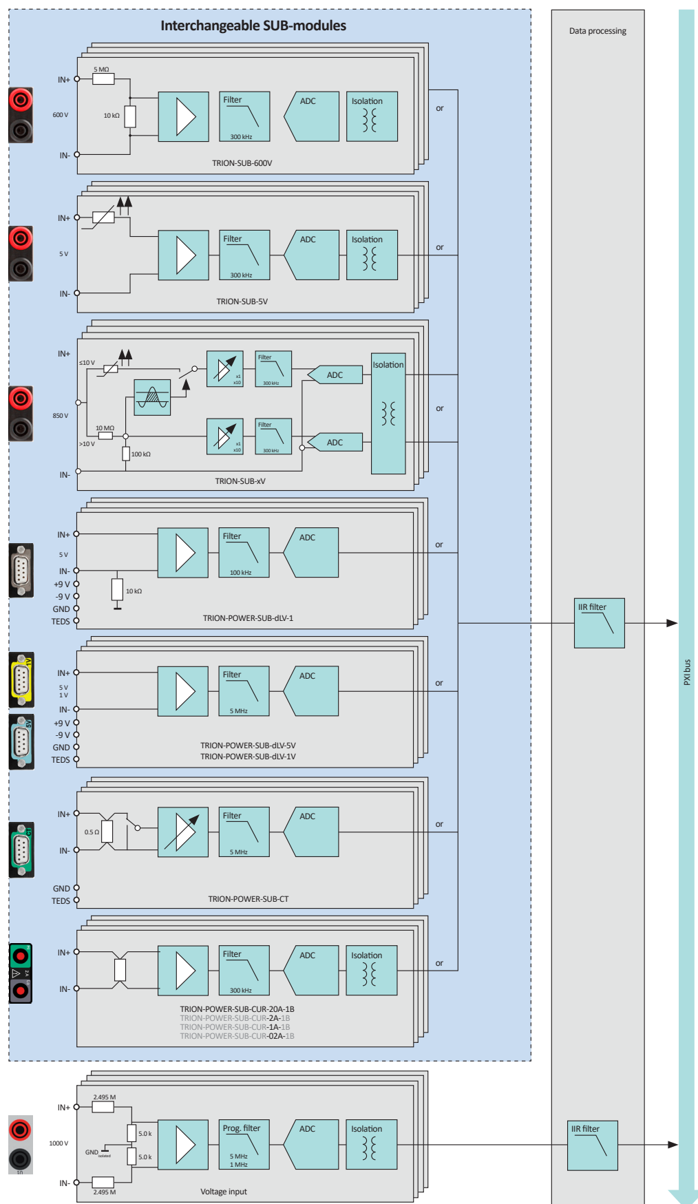
Fig. 147: Block diagram
