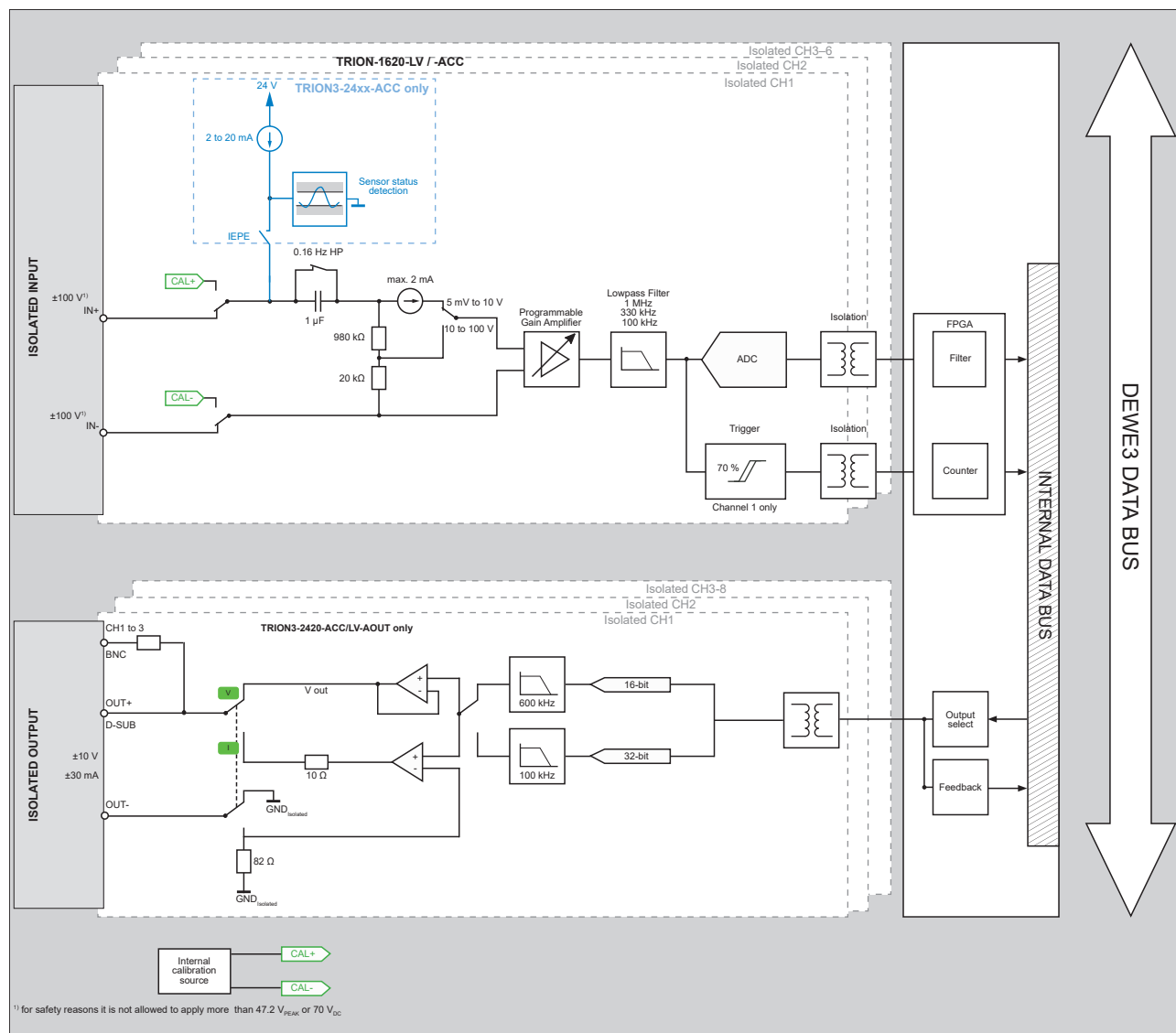
Fig. 80: Analog block diagram
