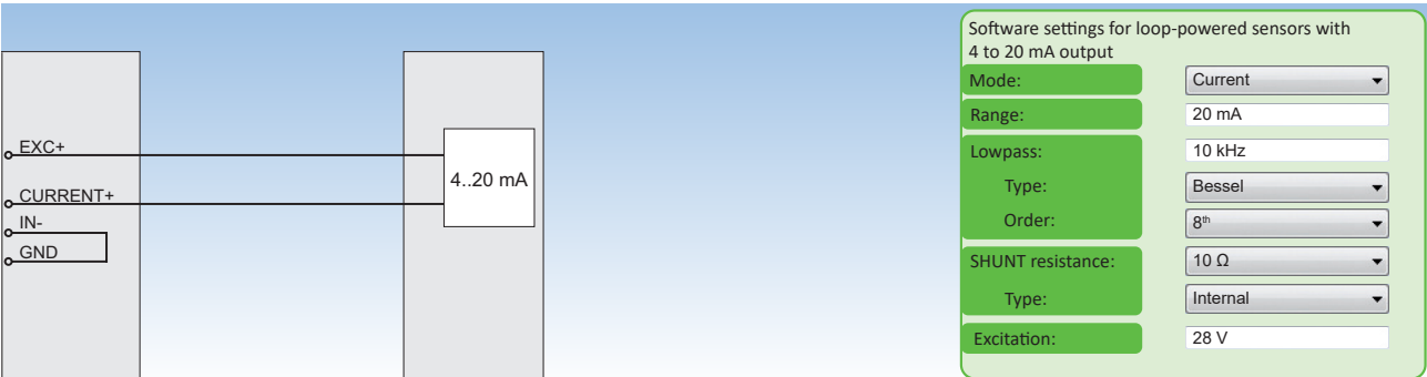
Fig. 107: Loop-powered sensors with 4 to 20 mA output
