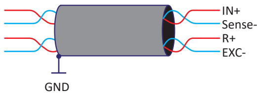
Fig. 130: Cables and shielding for full bridge, half bridge and voltage modes
