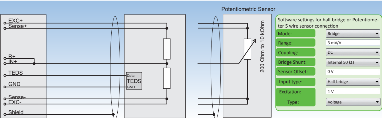
Fig. 123: Half bridge or Potentiometer 5-wire sensor connection
