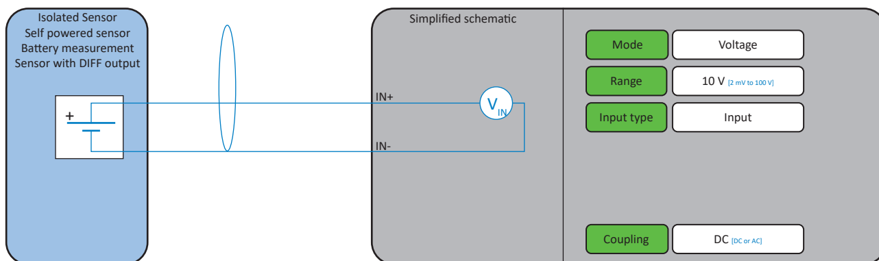
Fig. 85: Voltage measurement
