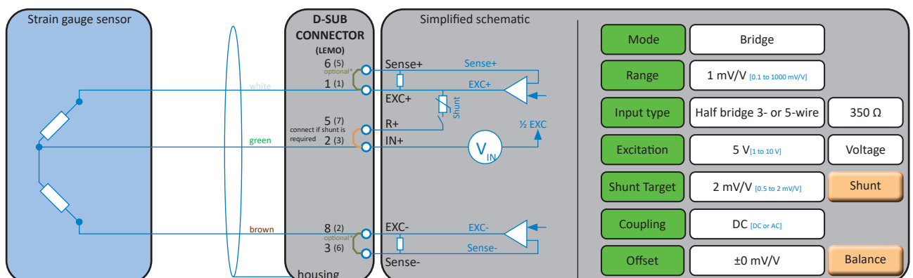
Fig. 40: Half bridge 3-wire
