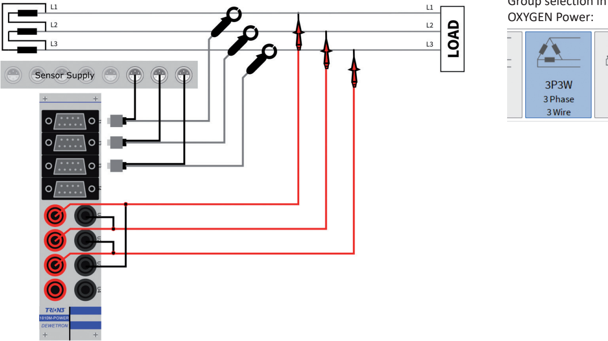
Fig. 159: Three phase (3P3W) without neutral line, using voltage output transducers
