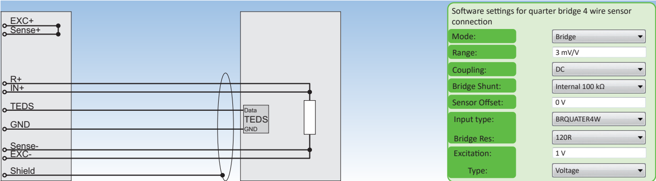
Fig. 126: Quarter bridge 4 wire sensor connection
