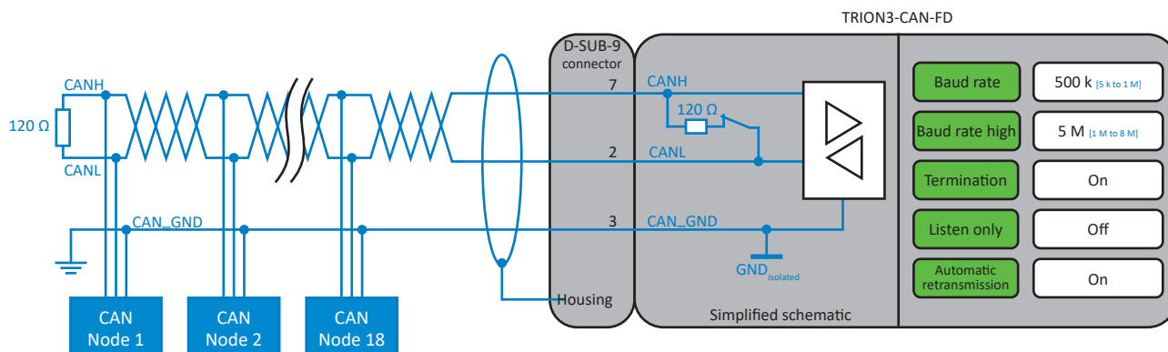
Fig. 219: Connecting sensors via CAN Bus
