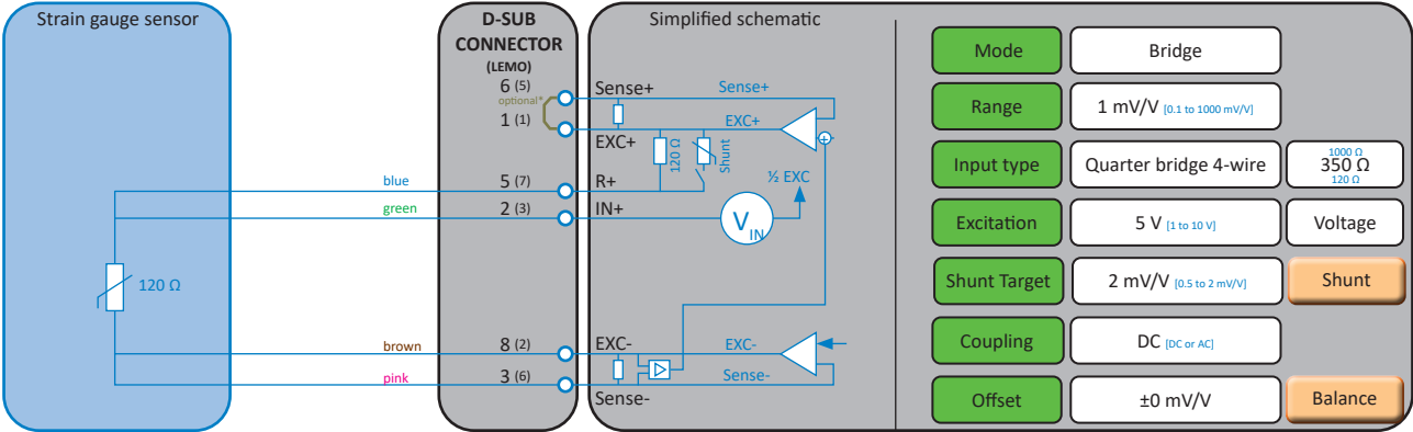
Fig. 41: Quarter bridge 4-wire
