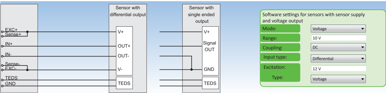
Fig. 119: Sensors with sensor supply and voltage output
