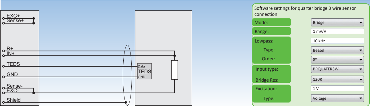
Fig. 65: Quarter bridge 3 wire sensor connection
