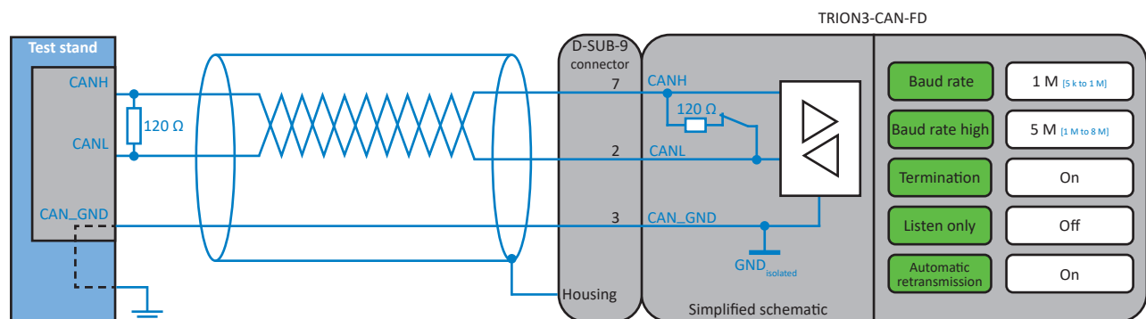
Fig. 221: Peer to peer
