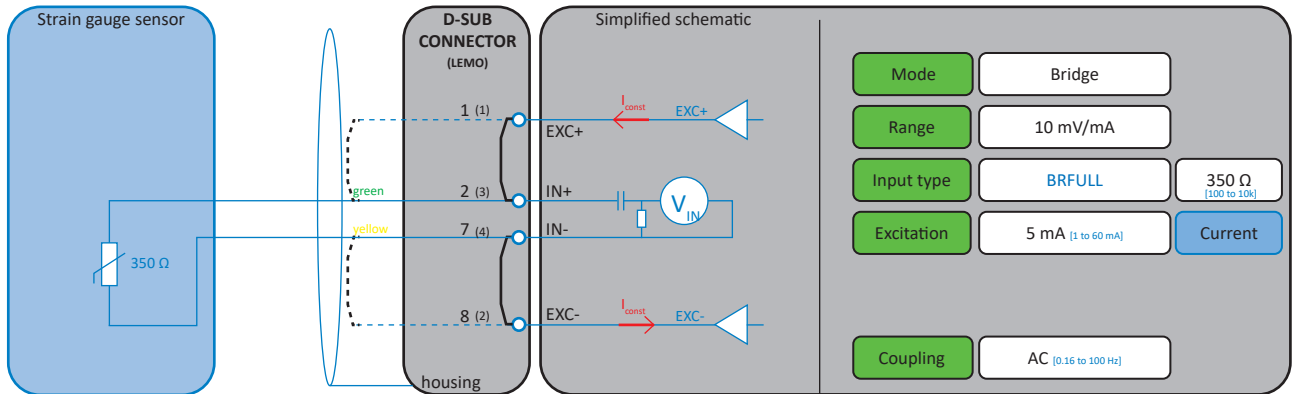
Fig. 44: Strain measurement with constant-current supply and AC coupling
