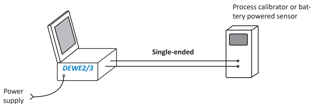
Fig. 136: Power supply / process calibrator or battery powered sensor
