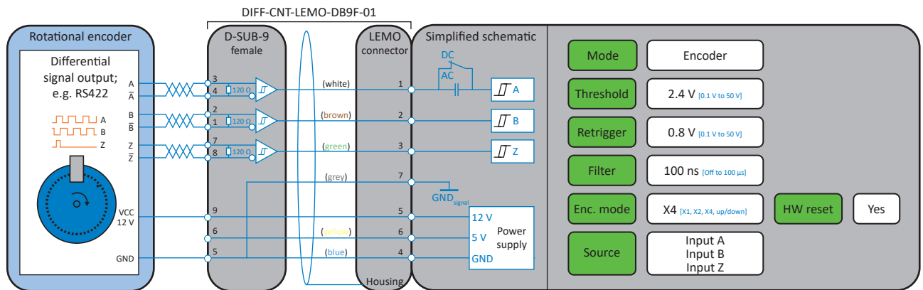
Fig. 200: Rotational encoder
