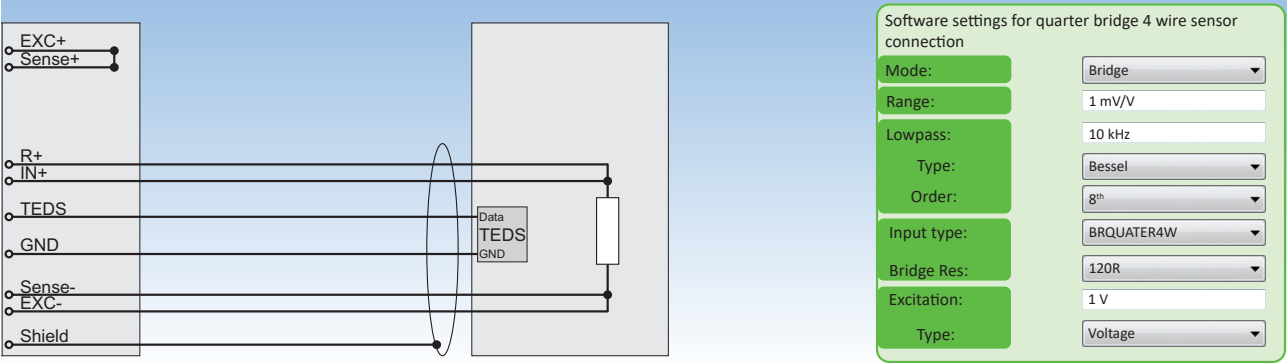
Fig. 66: Quarter bridge 4 wire sensor connection
