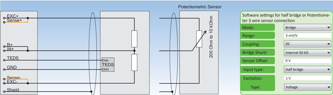
Fig. 124: Half bridge or Potentiometer 3 wire sensor connection
