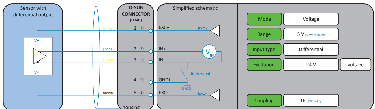
Fig. 29: Differential output sensor powered by the TRION module
