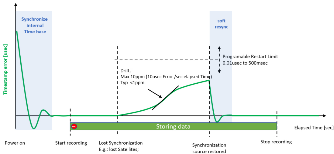
Fig. 187: Gapless recording
