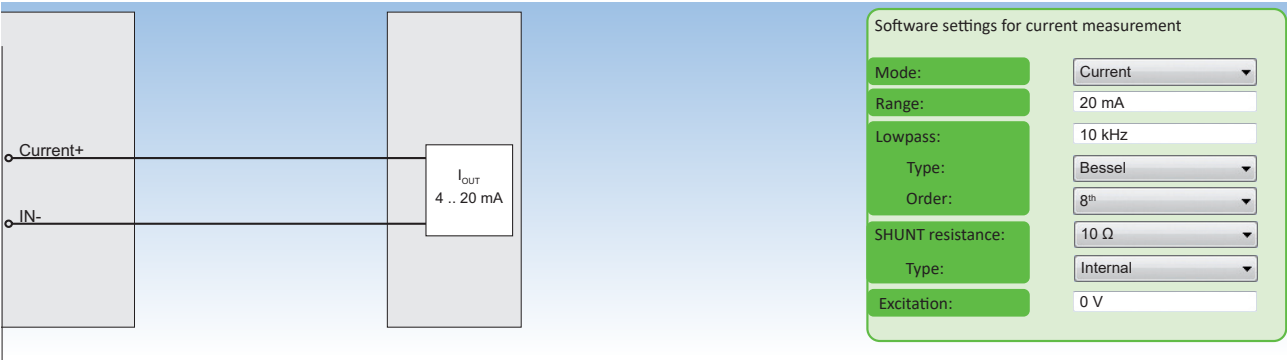
Fig. 105: Current measurement
