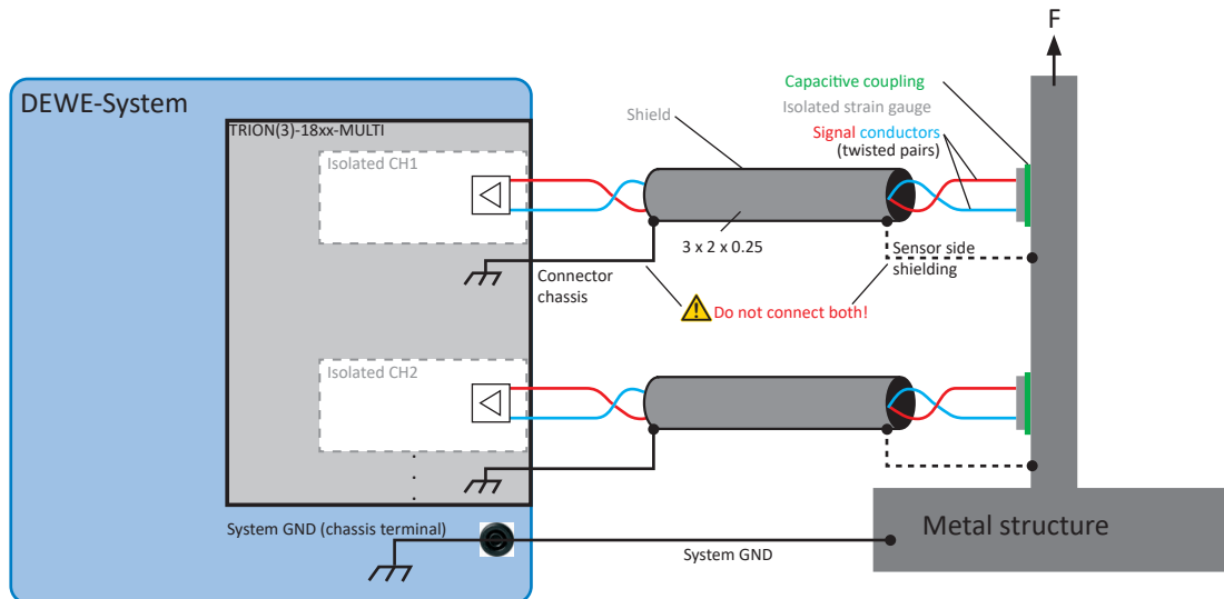
Fig. 55: Strain gauge measurement on a metal structure
