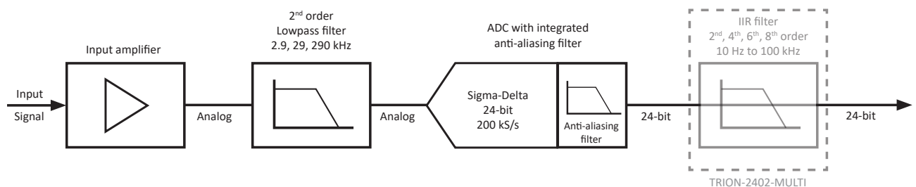
Fig. 7: TRION-2402 sample system architecture
