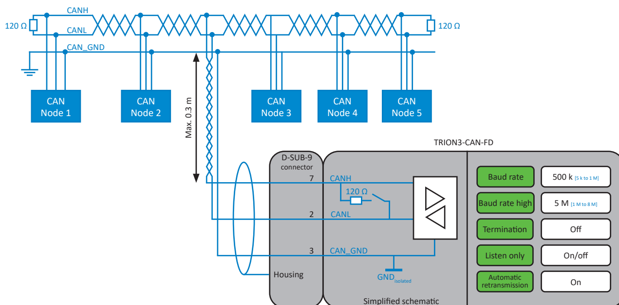
Fig. 218: Analyzing or monitoring a CAN bus
