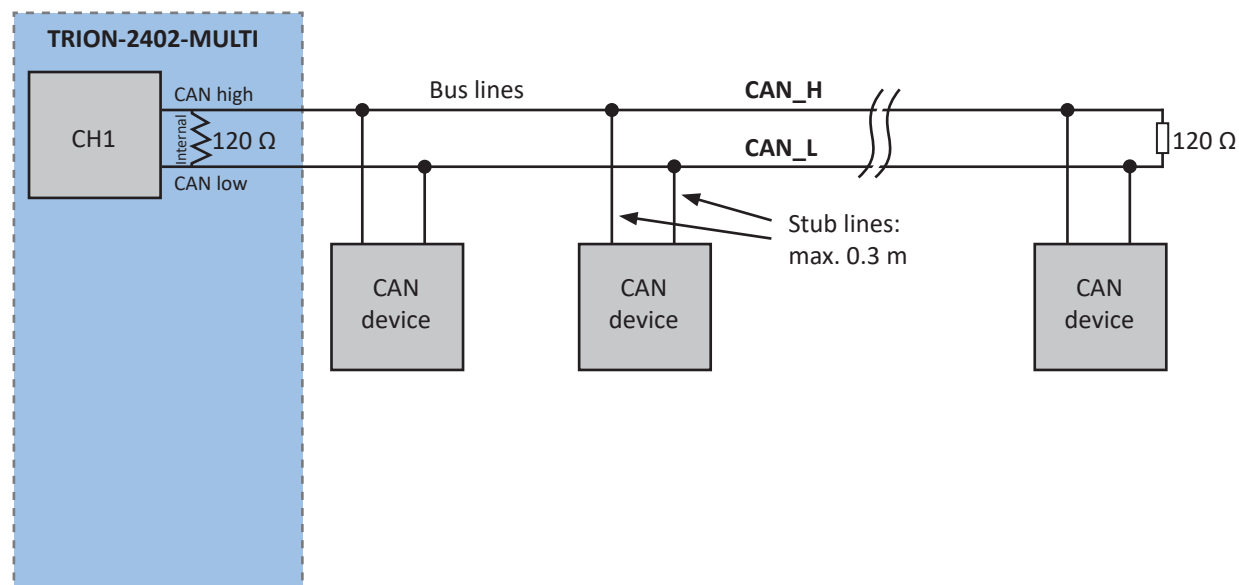
Fig. 70: CAN bus connection
