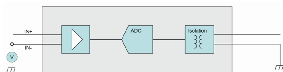
Fig. 242: Isolation voltage
