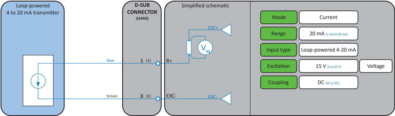
Fig. 32: Loop-powered 4 to 20 mA transmitter
