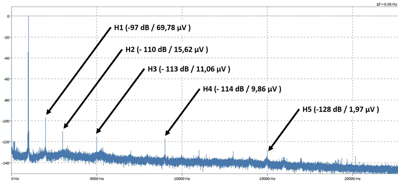
Fig. 238: THD measurement of TRION-1802/1600-dLV-32 (@50 kS/s) where U_f = 4.94 V equals 0 dB
