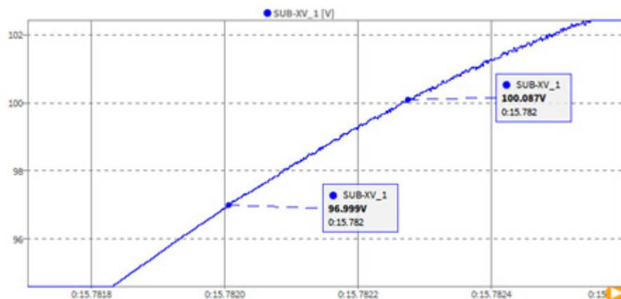
Fig. 232: TRION-SUB-XV auto ranging 100 V ↔ 1000 V switch over
