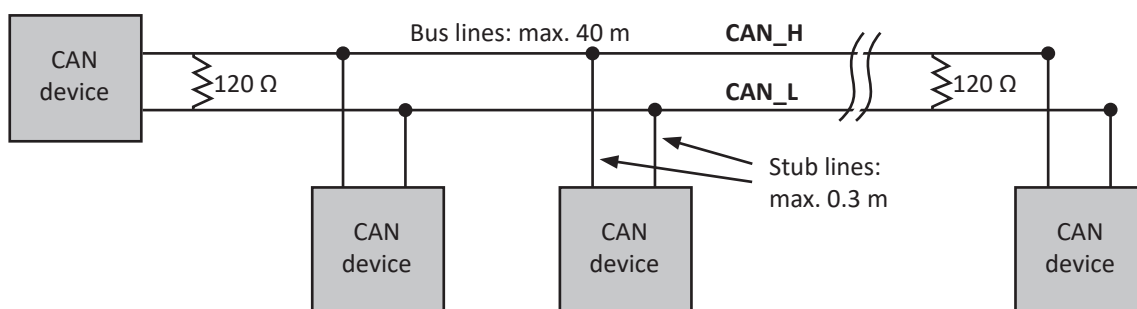
Fig. 225: High-speed CAN
