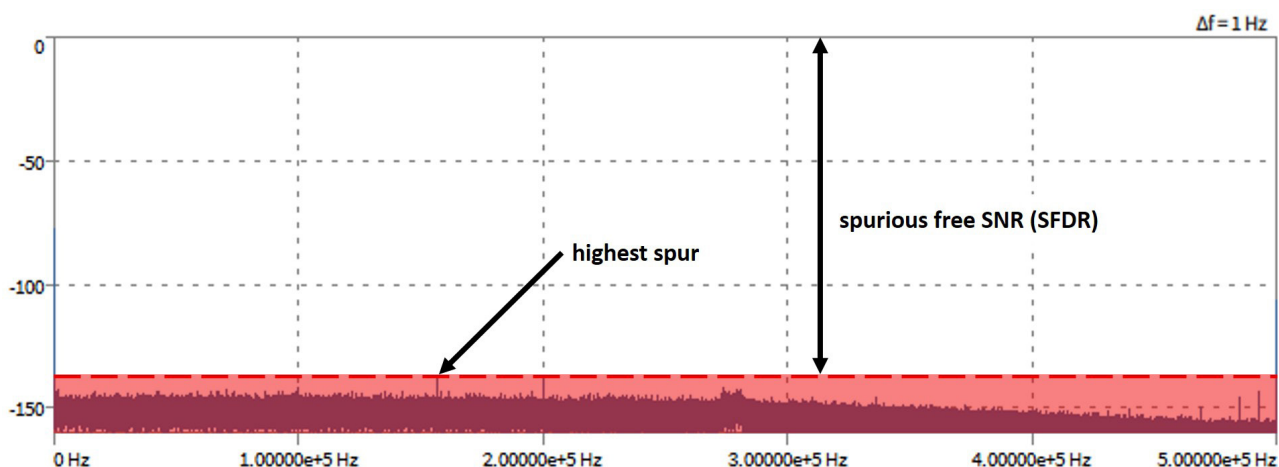
Fig. 236: SFDR in a FFT chart without input signal (DEWETRON)
