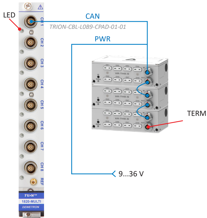
Fig. 56: Connecting XR modules to the TRION(3)-18xx-MULTI
