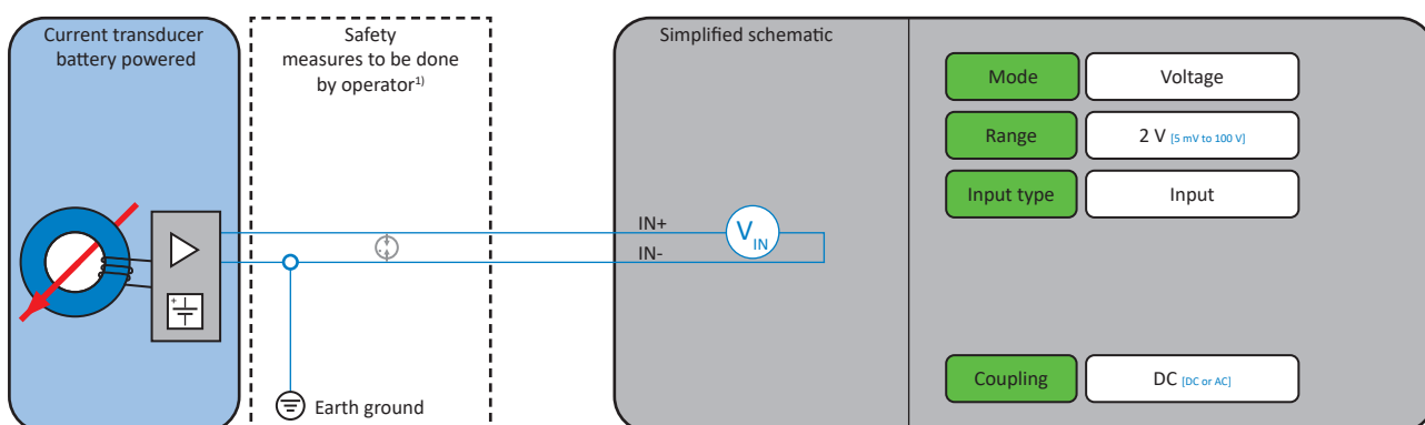
Fig. 86: Current transducer with voltage output
