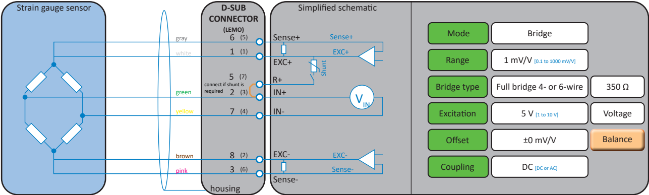
Fig. 34: Full bridge 6-wire
