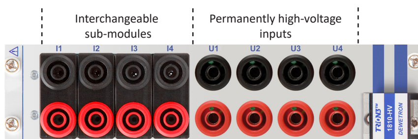
Fig. 142: Connection ports
