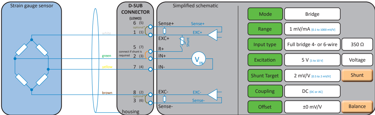
Fig. 36: Full bridge 4-wire
