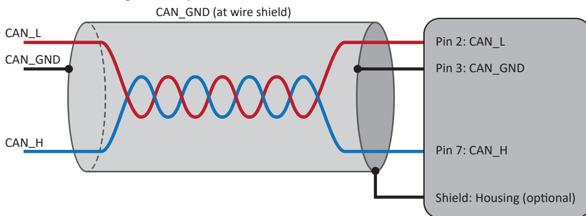
Fig. 222: Cabling for light industrial environment
