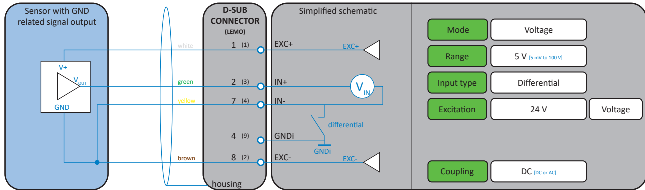
Fig. 30: Single-ended sensor powered by the TRION module
