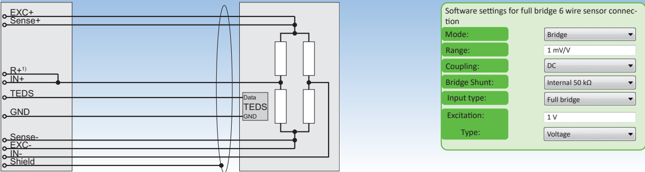
Fig. 121: Full bridge 6-wire sensor connection
