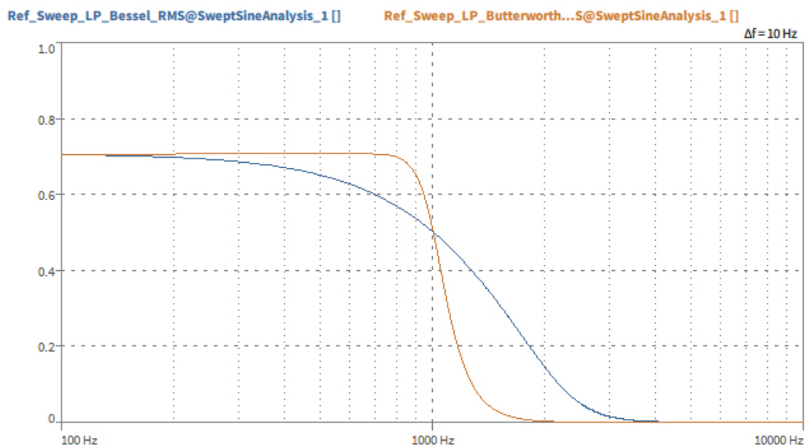
Fig. 155: Frequency response of filter with 1000 Hz cutoff frequency and 8th order
