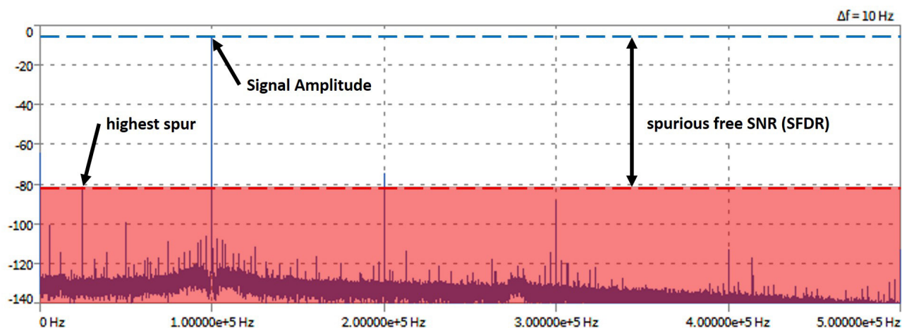
Fig. 235: SFDR in a FFT chart with input signal (alternative method)
