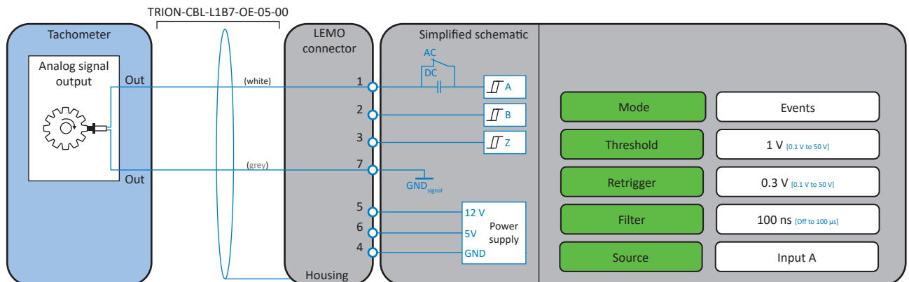
Fig. 197: Event counting (analog output)
