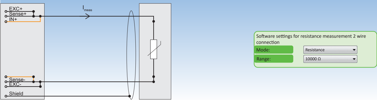
Fig. 127: Resistance and RTD measurement 2 wire connection
