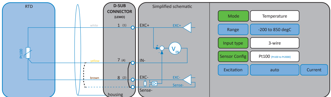
Fig. 48: RTD 3-wire temperature measurement
