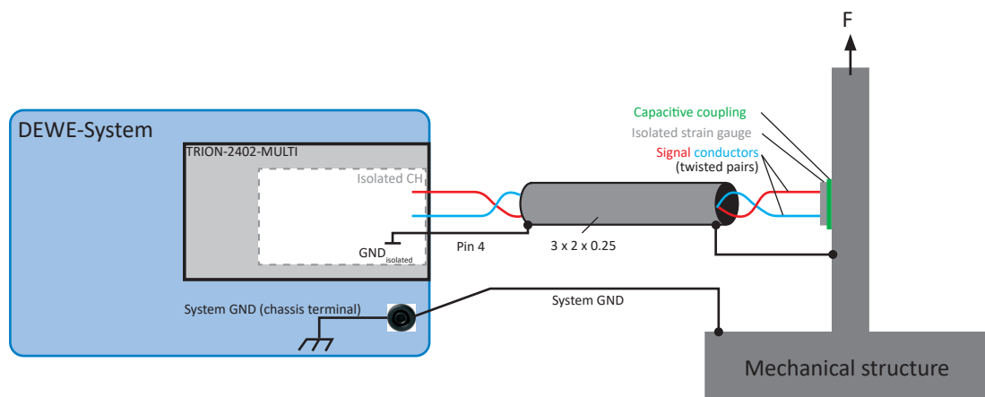
Fig. 73: Strain gauge measurement on a metal structure
