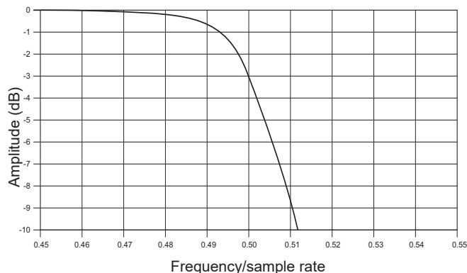
Input frequency response near the cut-off
