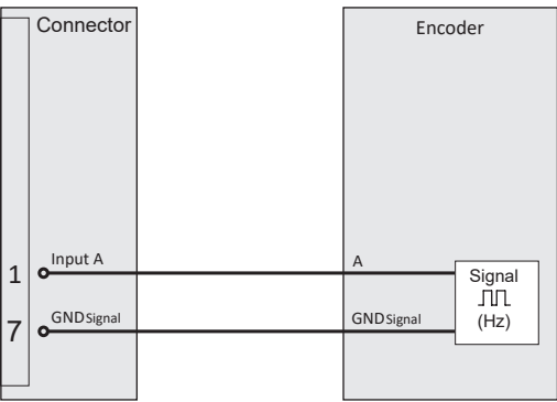
Fig. 181: Non-supplied sensor connection
