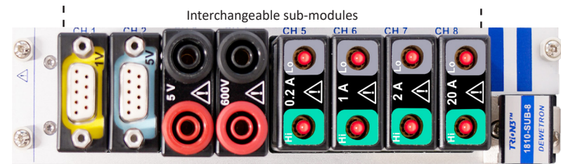
Fig. 169: Connection ports
