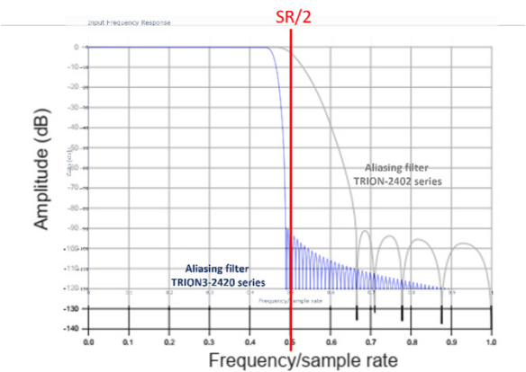
Fig. 79: Transfer function of aliasing filter at 100 kS/s
