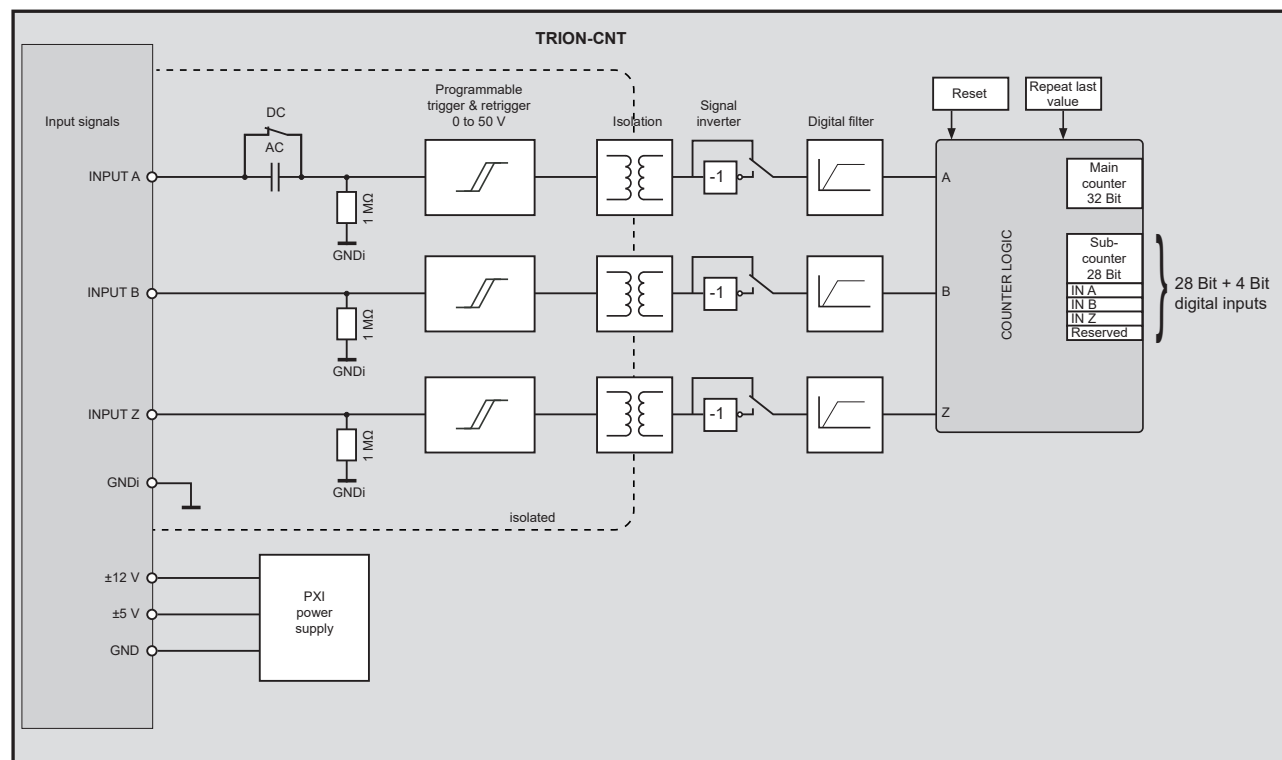
Fig. 203: Block diagram
