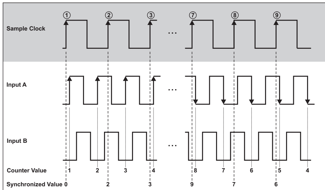
Fig. 211: Quadrature Encoder X1 Mode
