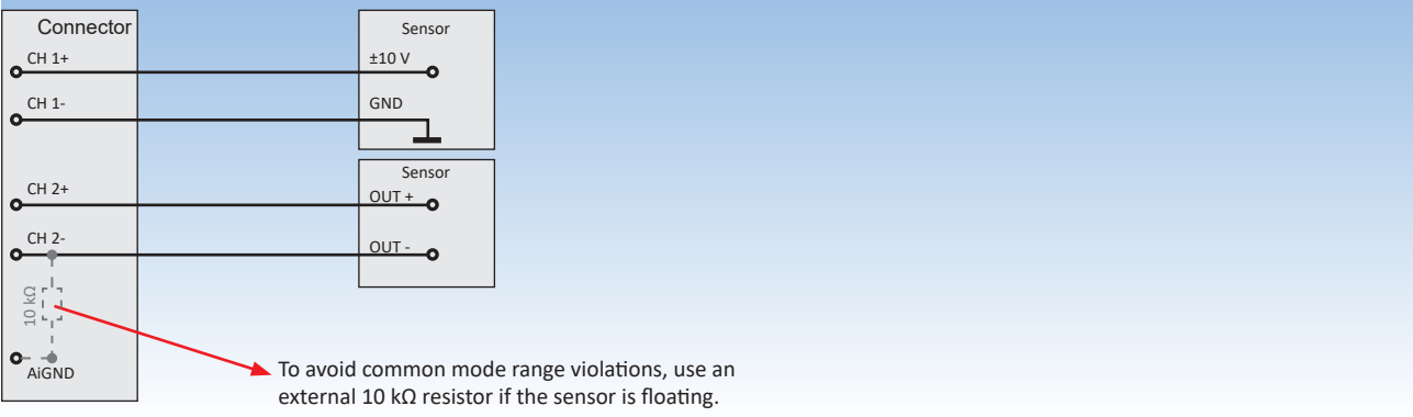
Fig. 115: Differential input
