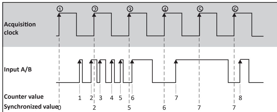
Fig. 207: Event counting
