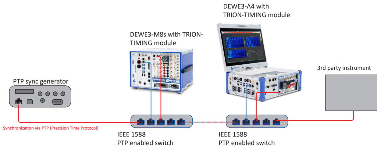
Fig. 191: Typical topology
