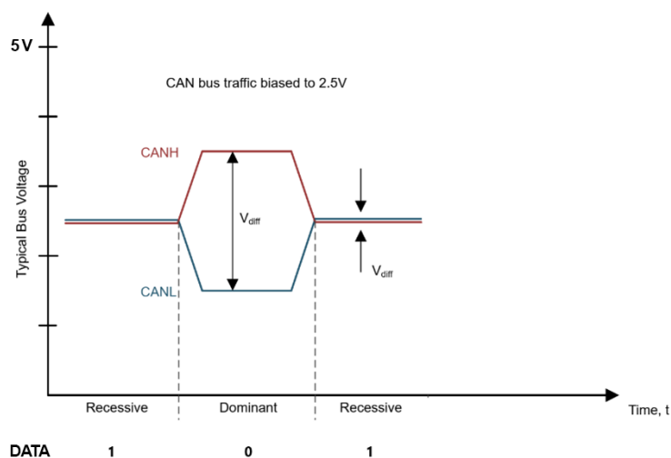
Fig. 217: CAN signal
