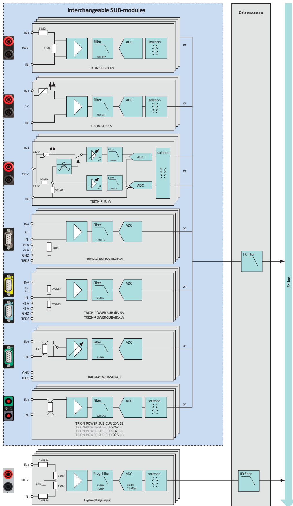
Fig. 156: Block diagram
