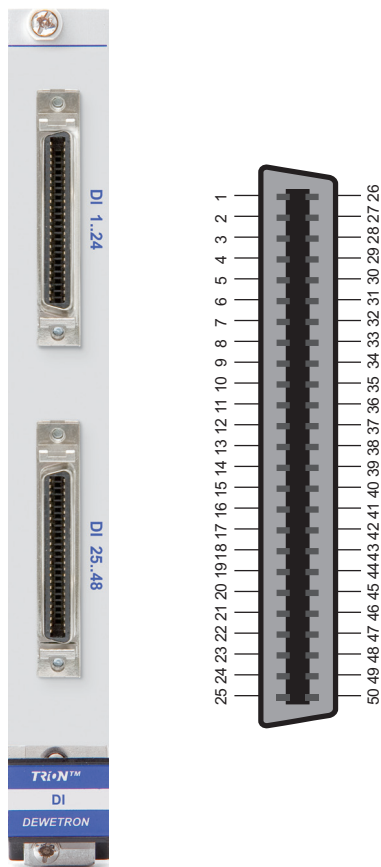
Fig. 229: 50-pin mini-centronics socket
