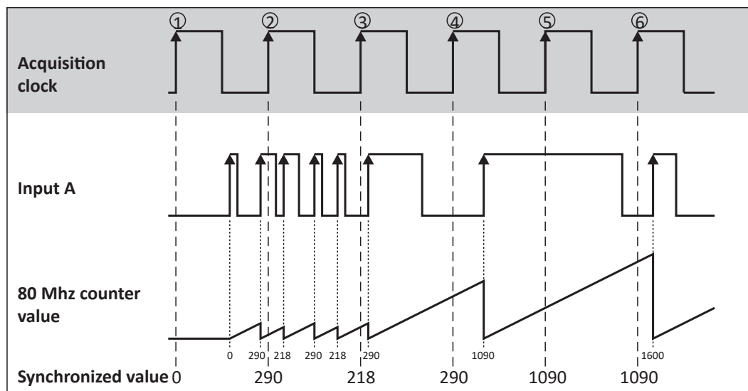
Fig. 208: Period time measurement
