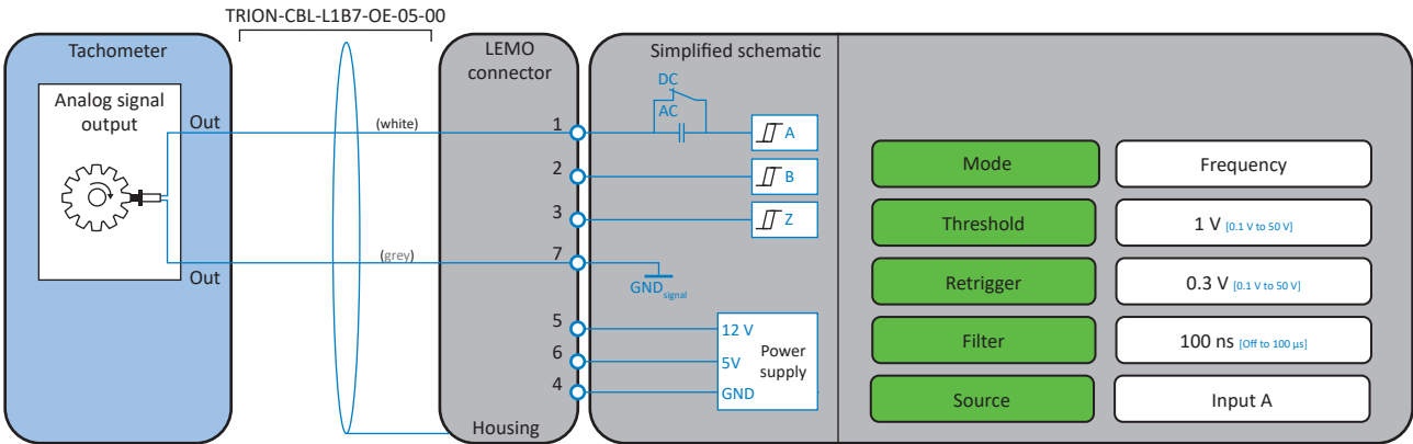
Fig. 198: Frequency measurement (analog output)
