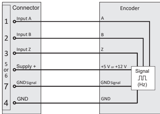
Fig. 180: Supplied sensor connection
