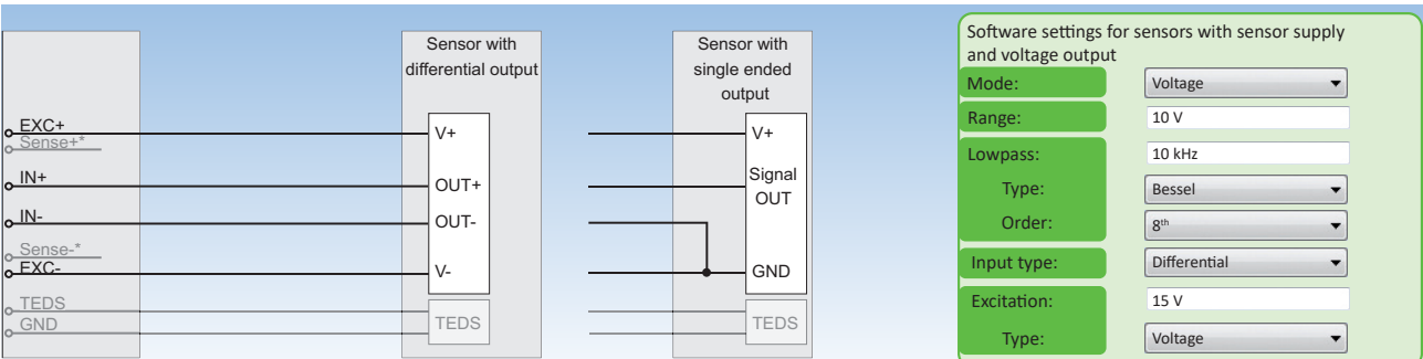
Fig. 59: Sensors with sensor supply and voltage output
