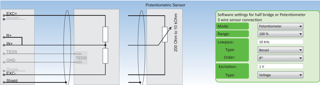
Fig. 64: Half bridge or Potentiometer 3 wire sensor connection
