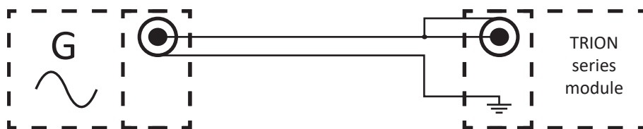
Fig. 239: Schematic circuit diagram of CMRR measurement
