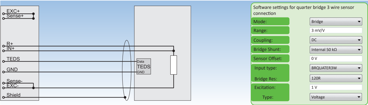
Fig. 125: Quarter bridge 3 wire sensor connection
