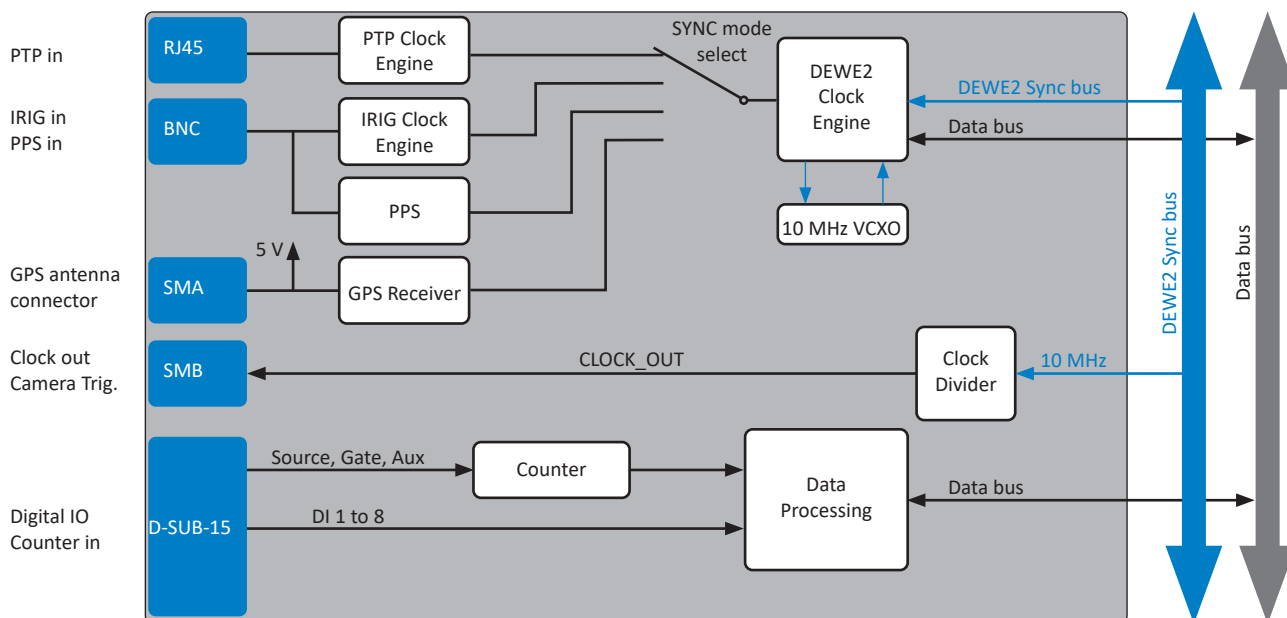
Fig. 183: Signal routing
