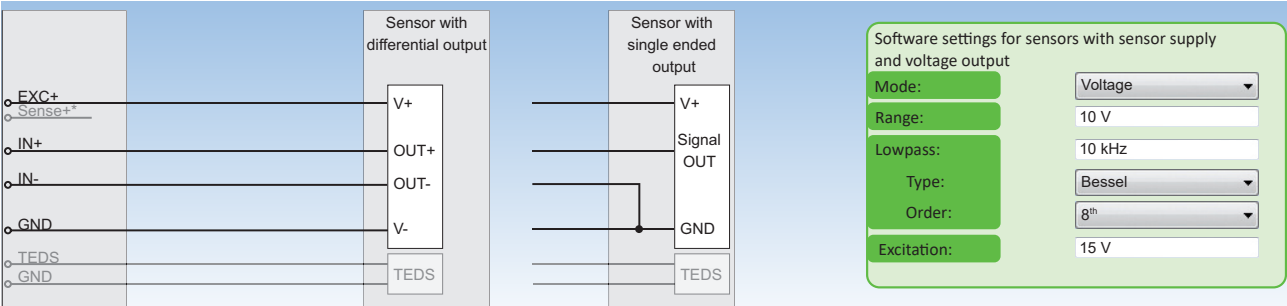
Fig. 104: Sensors with sensor supply and voltage output
