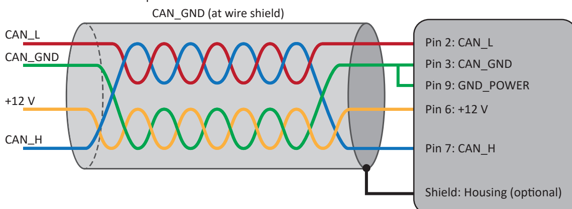
Fig. 224: Cabling for sensors with power supply
