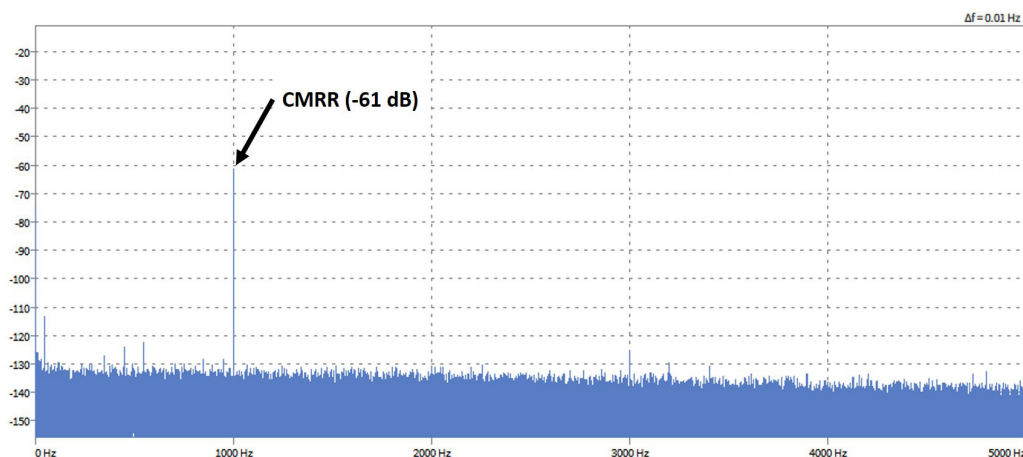
Fig. 240: Measurement of CMRR in FFT chart of TRION-1620-ACC (>2 V range @ 1 kHz)
