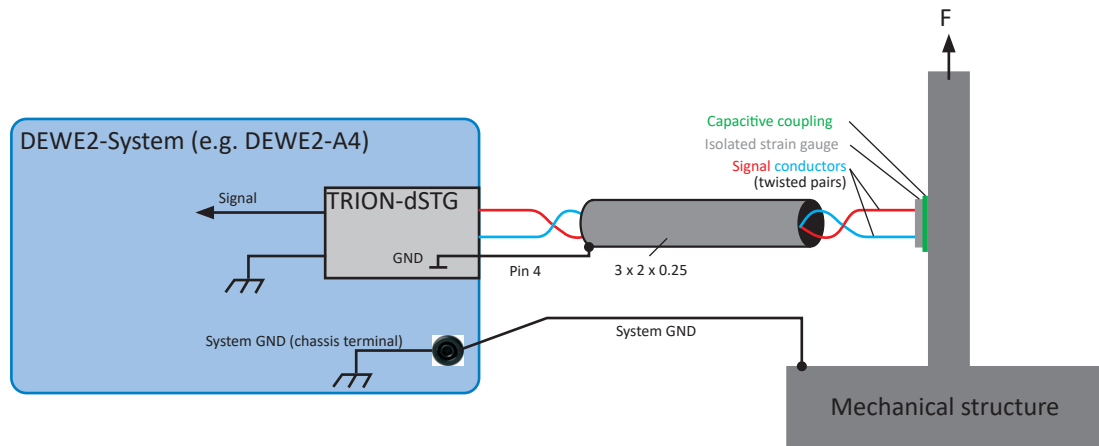
Fig. 131: Strain gauge measurement
