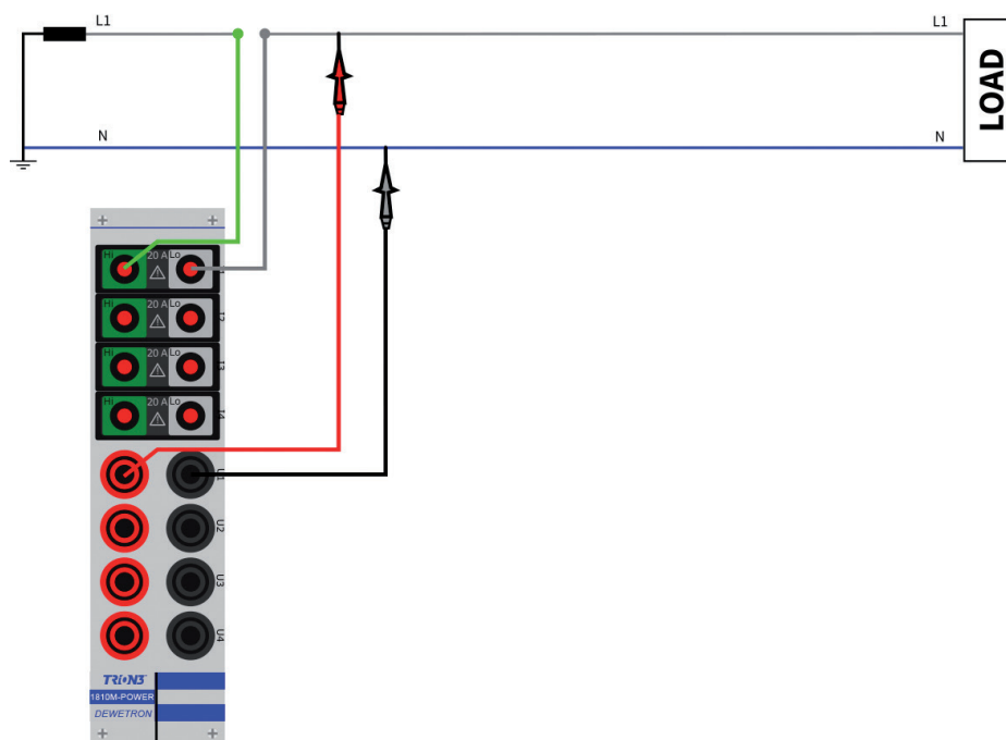
Fig. 161: One phase (1P2W)
