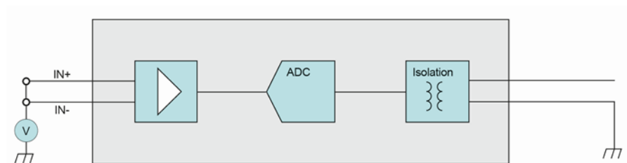
Fig. 245: Common mode voltage
