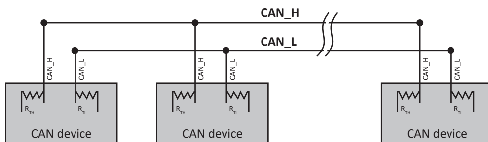
Fig. 226: Low-speed / fault-tolerant CAN
