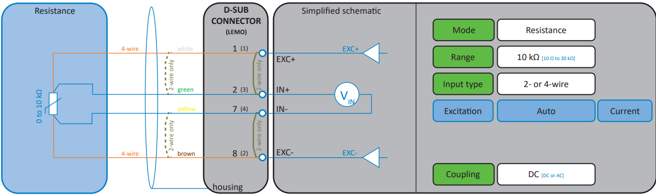
Fig. 46: Resistance measurement
