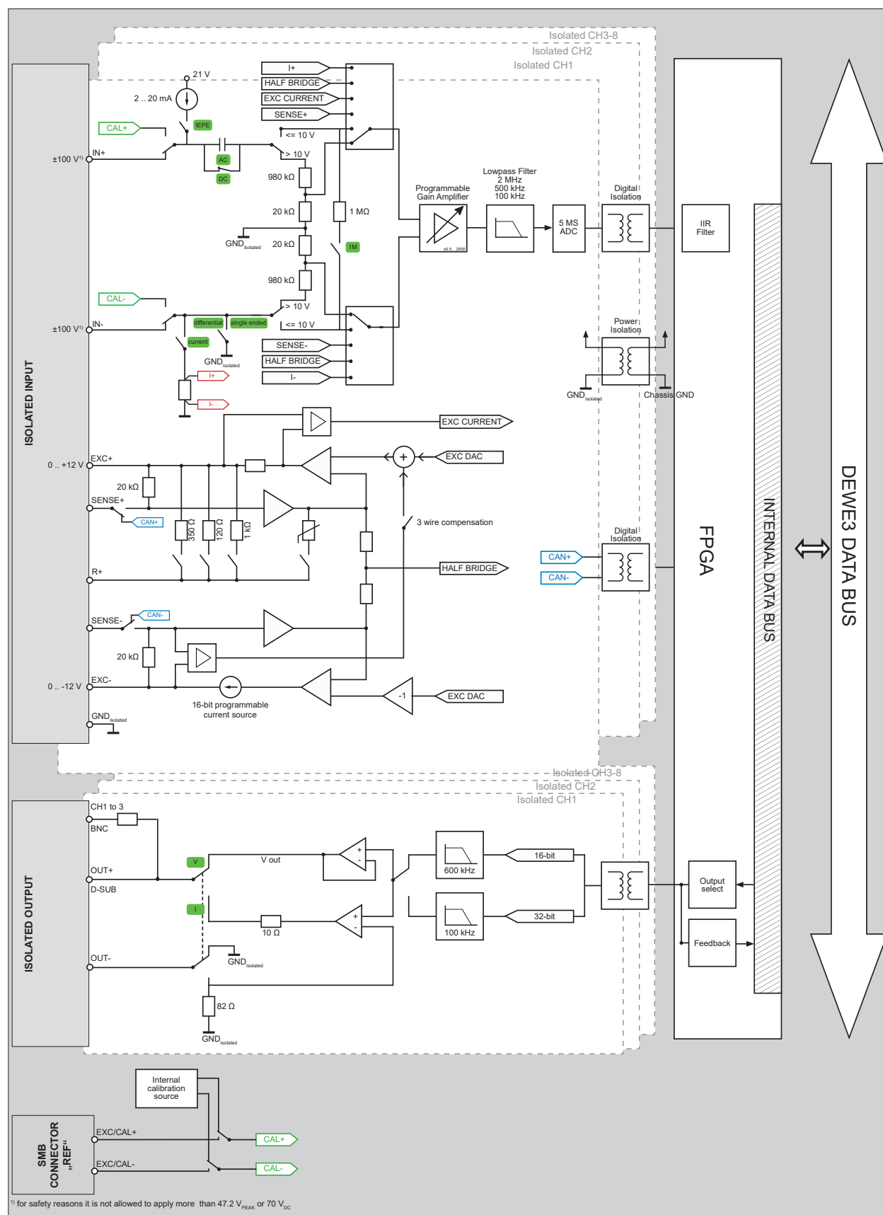
Fig. 24: Analog block diagram
