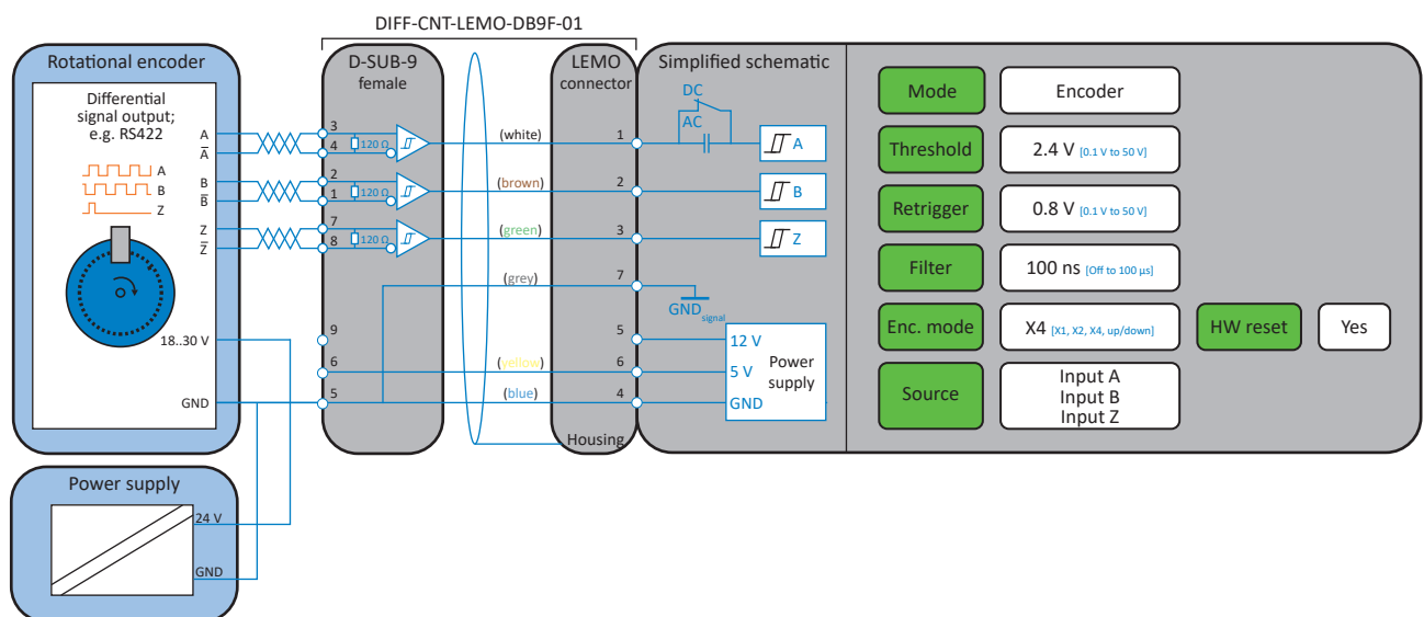
Fig. 201: Rotational encoder externally powered
