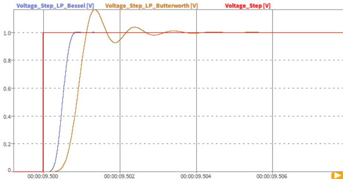
Fig. 154: Step response of filter with 1000 Hz cutoff frequency and 8th order.
