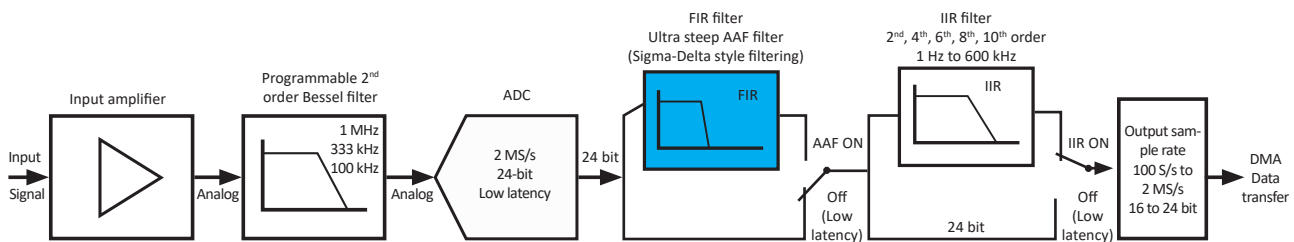
Fig. 78: Sample system architecture
