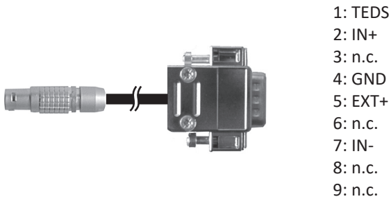
Fig. 99: TRION-CBL-L1B8-D9-0.5-01
