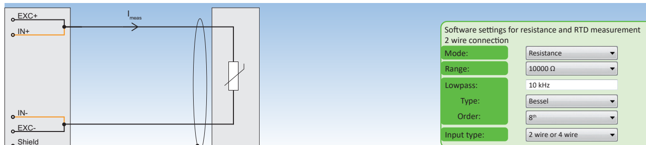
Fig. 67: Resistance and RTD measurement 2 wire connection
