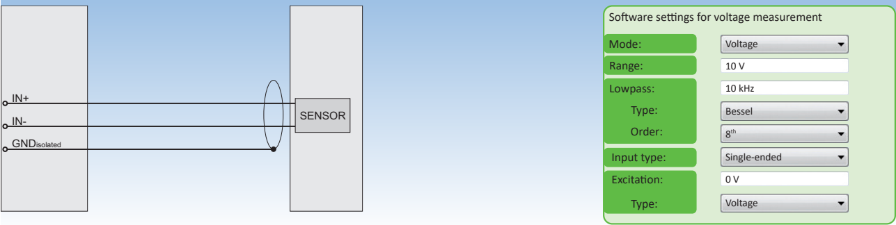
Fig. 58: Voltage measurement
