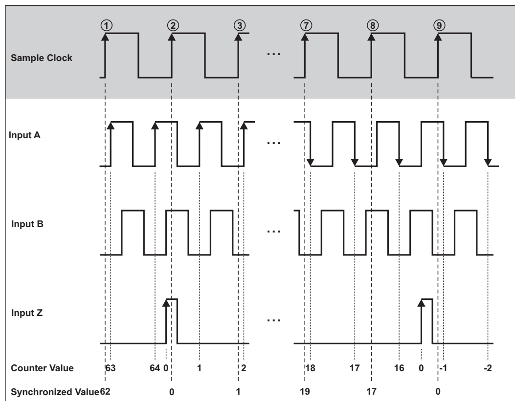
Fig. 214: Quadrature Encoder with channel Z
