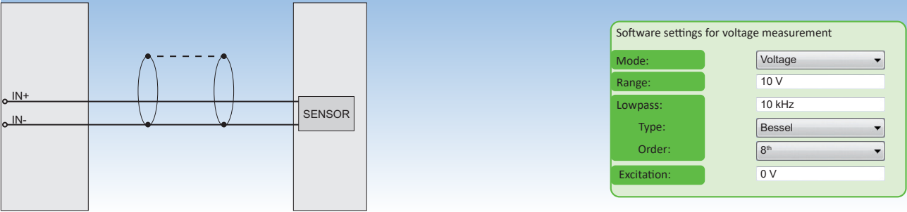
Fig. 93: Voltage measurement
