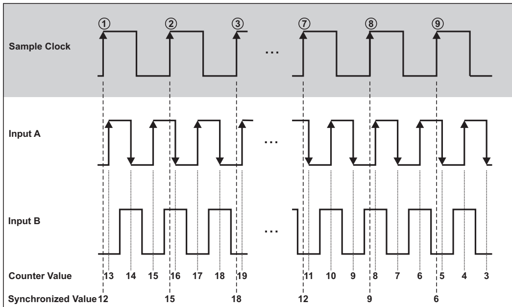
Fig. 212: Quadrature Encoder X2 Mode
