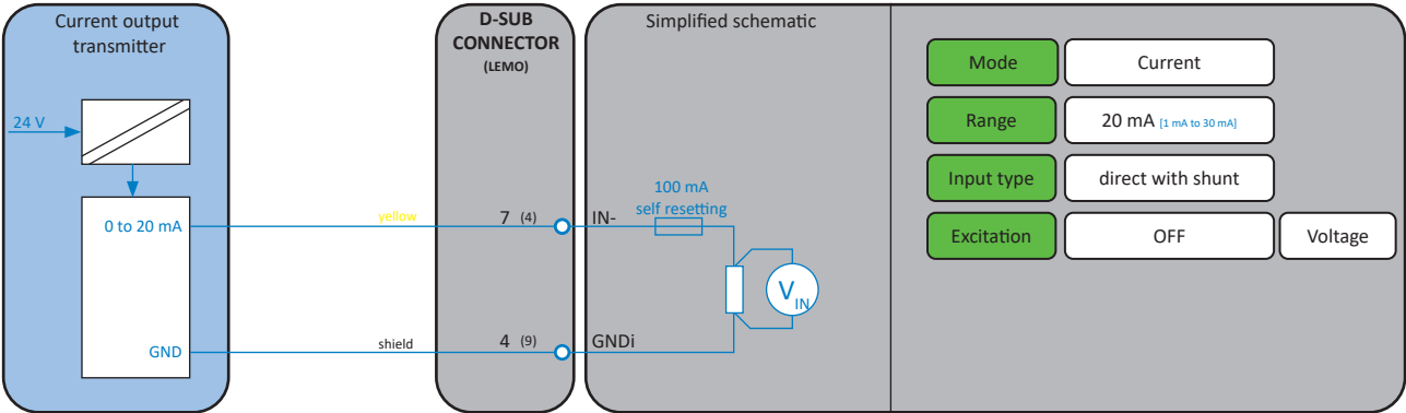
Fig. 33: Current measurement (with externally powered transmitter)
