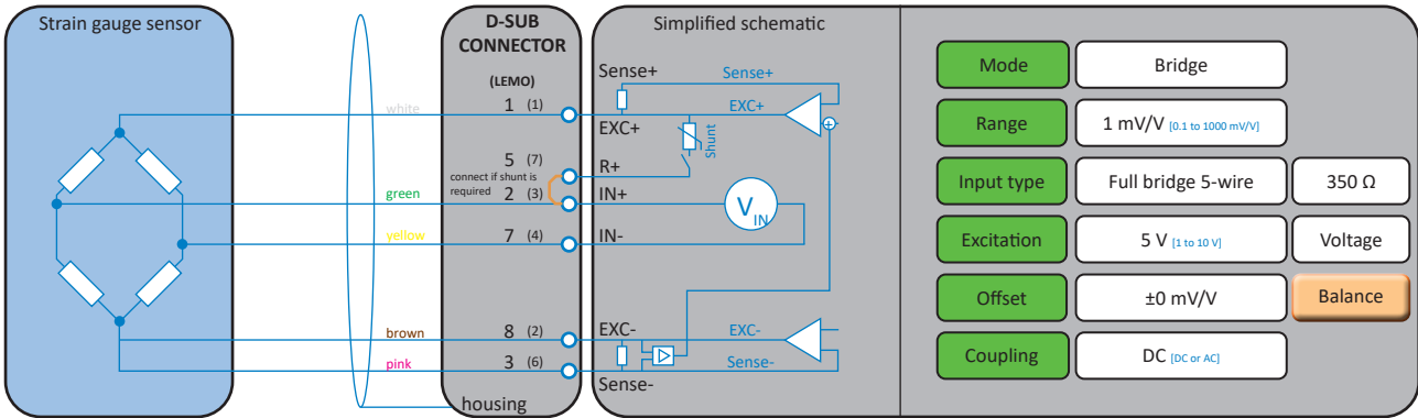
Fig. 35: Full bridge 5-wire
