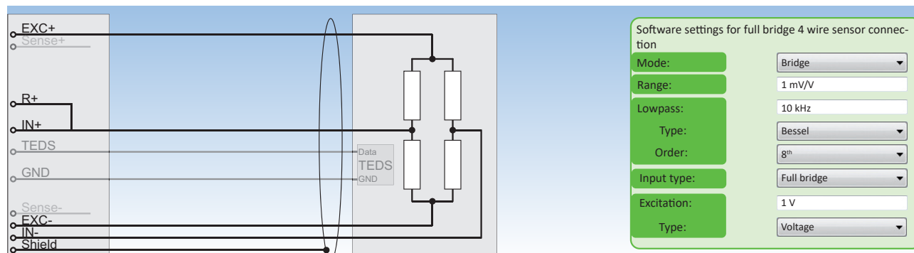
Fig. 62: Full bridge 4-wire sensor connection
