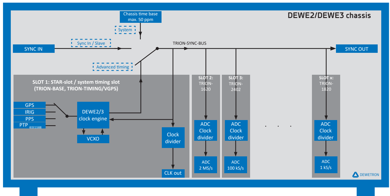
Fig. 18: DEWE chassis functional overview
