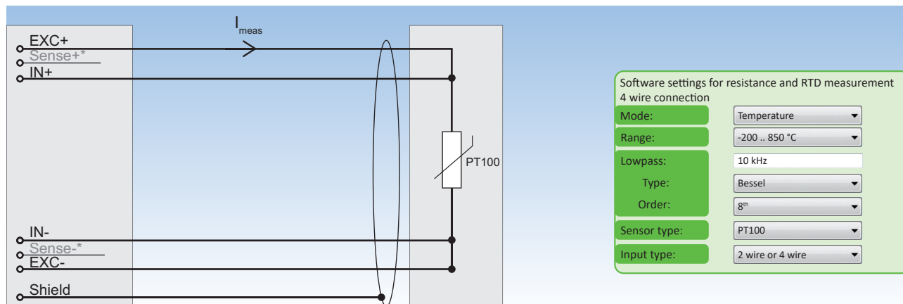
Fig. 69: Resistance and RTD measurement 4 wire connection
