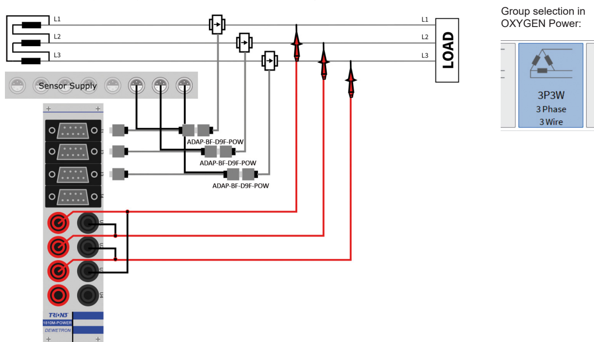
Fig. 158: Three phase (3P3W) without neutral line, using current output transducer
