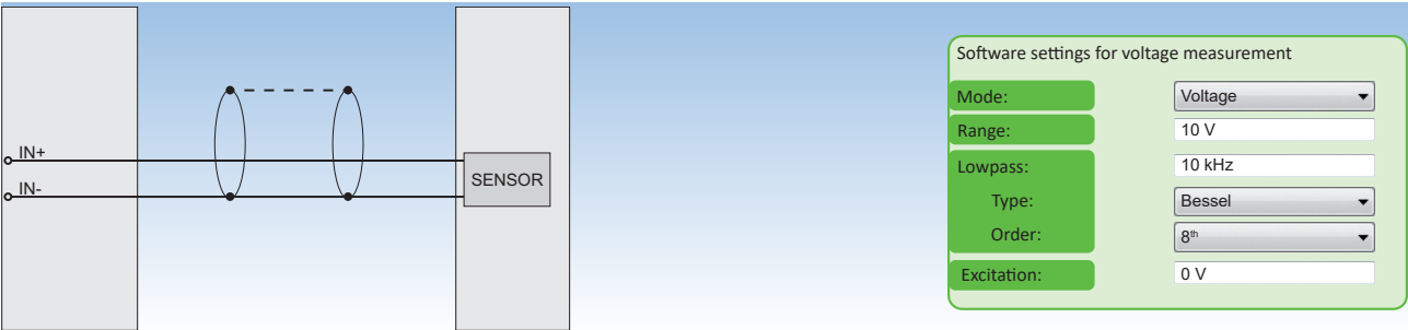
Fig. 103: Voltage measurement
