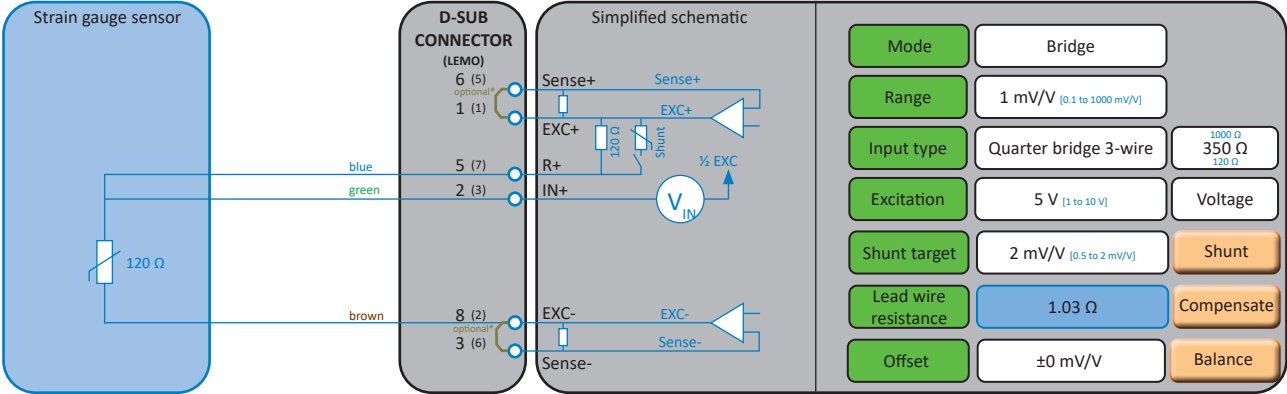
Fig. 42: Quarter bridge 3-wire
