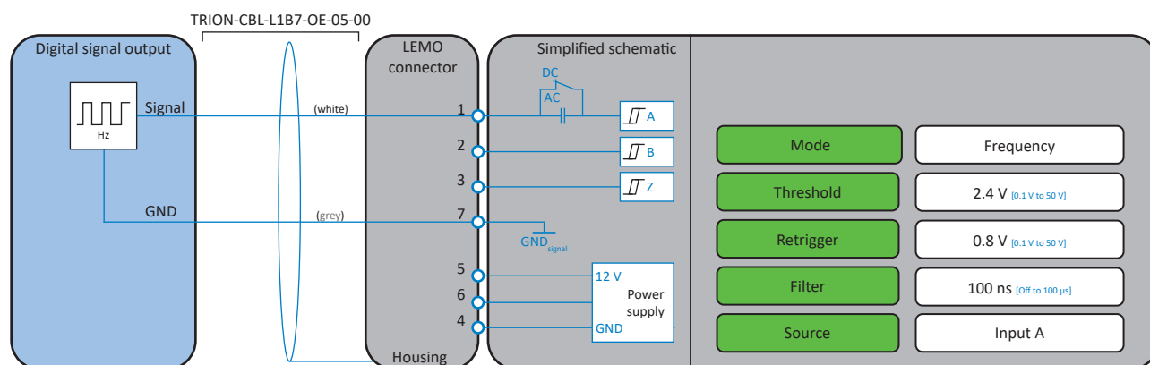
Fig. 195: Frequency (digital output)
