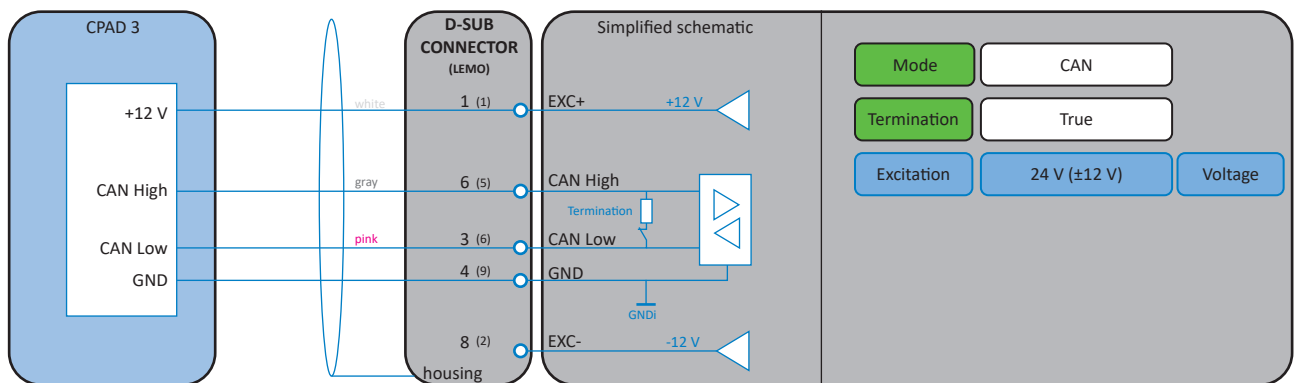
Fig. 52: CAN
