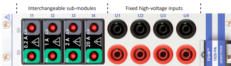
Fig. 148: Connection ports
