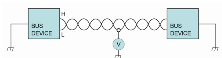
Fig. 247: Bus pin fault protection
