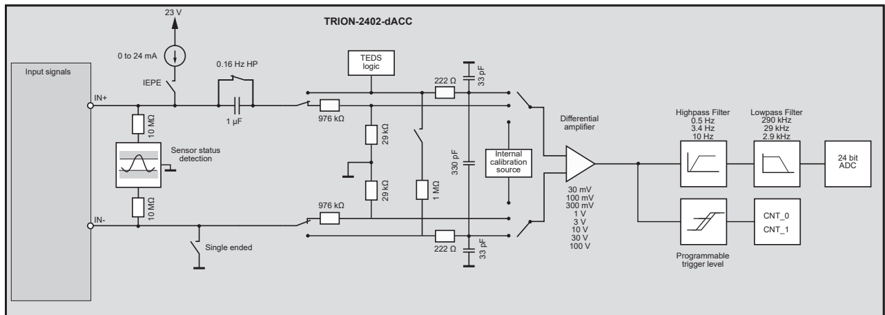
Fig. 133: Block diagram
