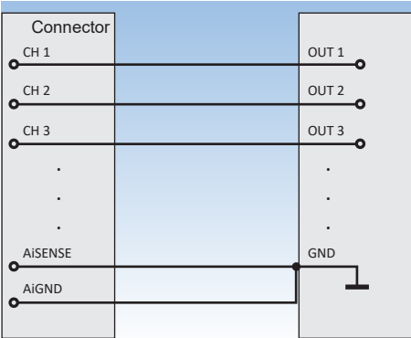
Fig. 114: Single-ended
