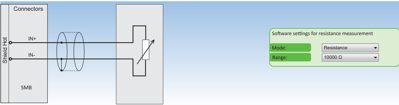
Fig. 141: Resistance
