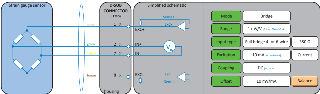
Fig. 37: Full bridge 4-wire with constant current excitation
