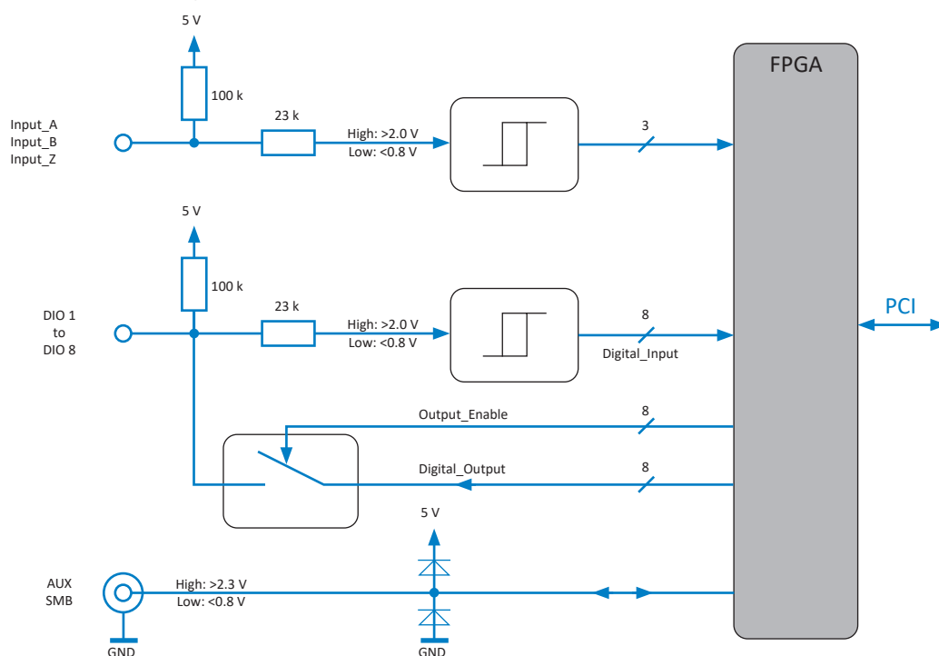
Fig. 185: Counter and digital I/O
