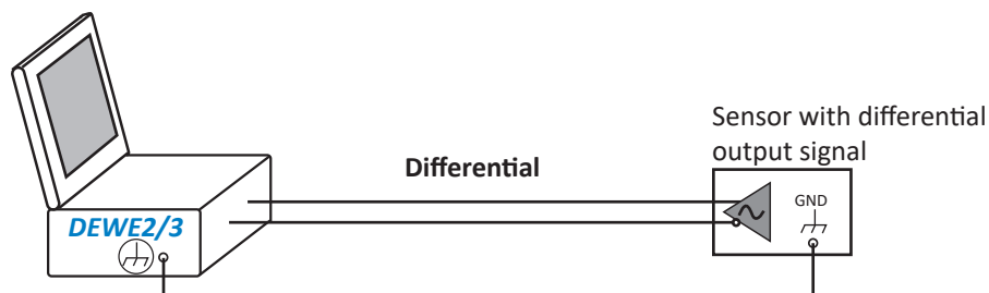
Fig. 137: Sensor with differential output signal
