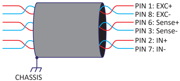
Fig. 54: Cables and shielding
