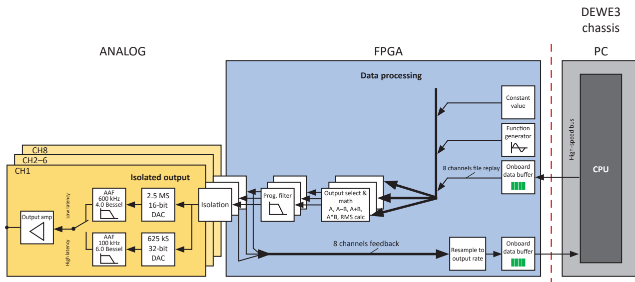
Fig. 179: Signal path
