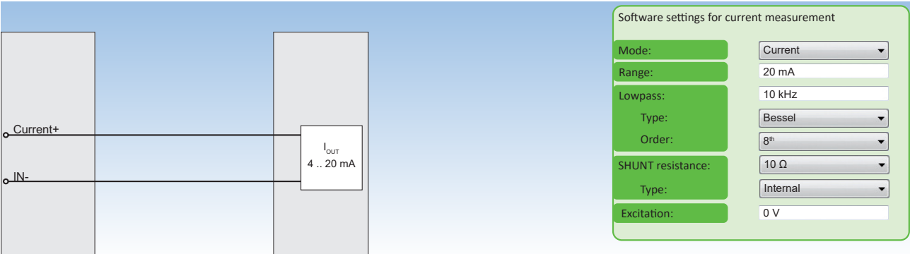
Fig. 95: Current measurement
