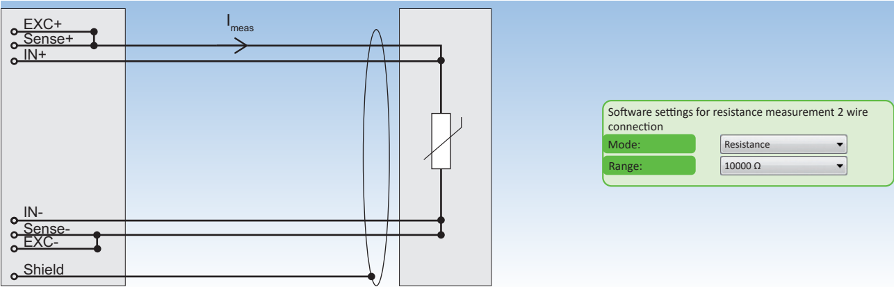
Fig. 128: Resistance and RTD measurement 4 wire connection
