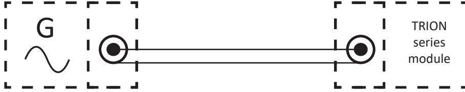
Fig. 237: Schematic circuit diagram of THD measurement
