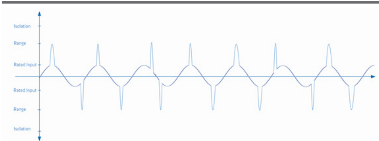
Fig. 244: Relation between rated input, input ranges and isolation voltage
