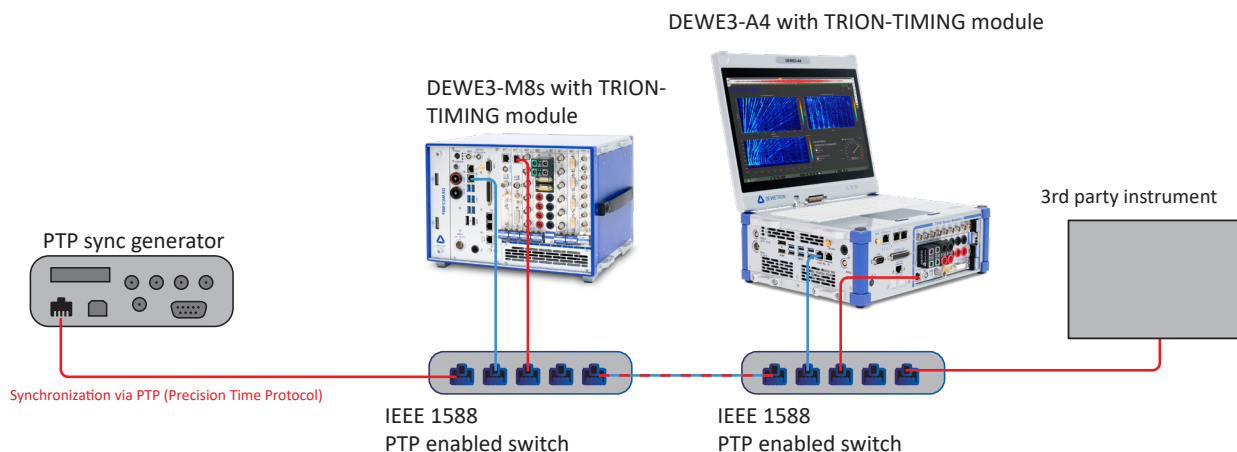
Fig. 186: Typical topology
