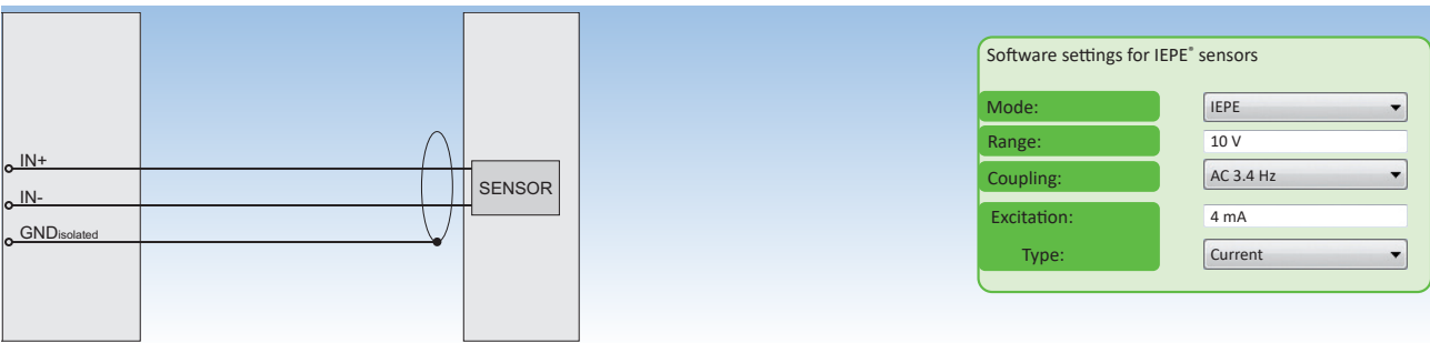
Fig. 120: IEPE® sensor
