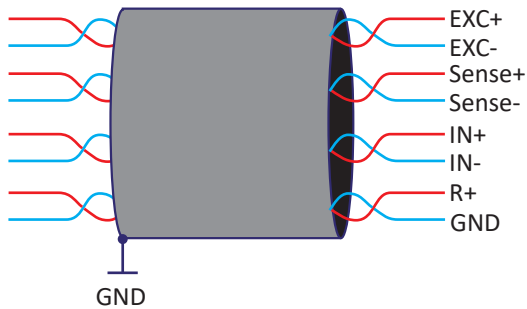
Fig. 129: Cables and shielding for full bridge, half bridge and voltage modes
