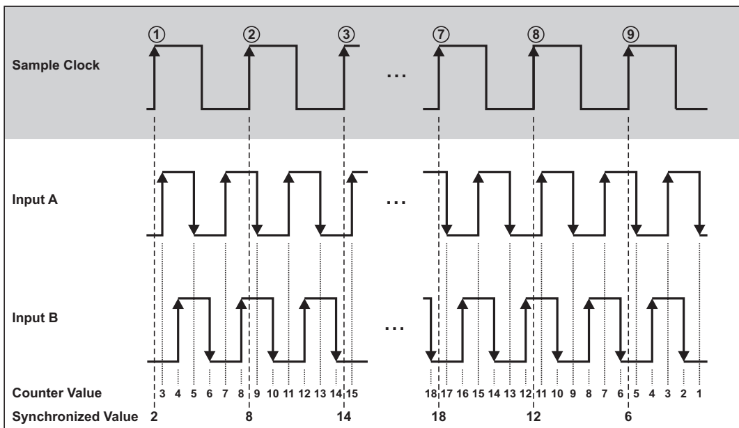
Fig. 213: Quadrature Encoder X4 Mode
