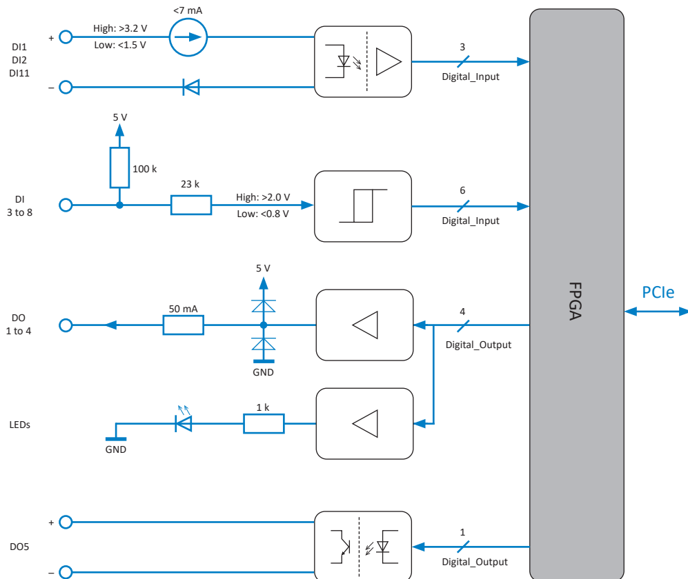
Fig. 82: Digital block diagram
