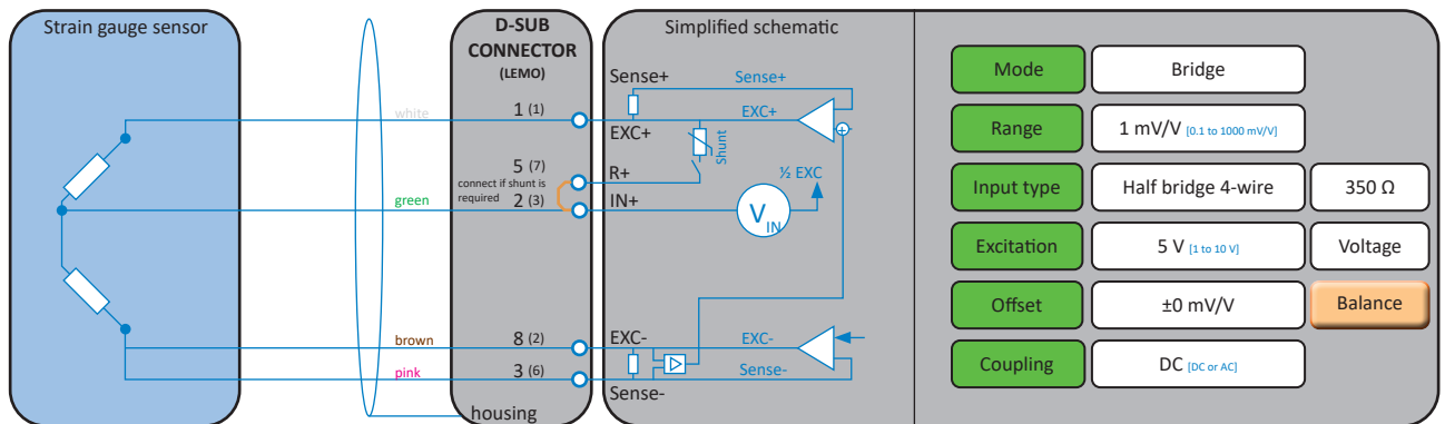
Fig. 39: Half bridge 4-wire
