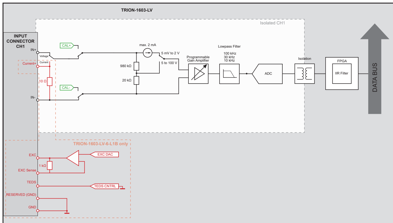
Fig. 102: Base block diagram of the TRION-1603-LV module
