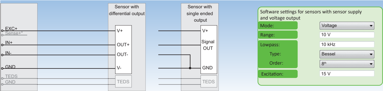
Fig. 94: Sensors with sensor supply and voltage output
