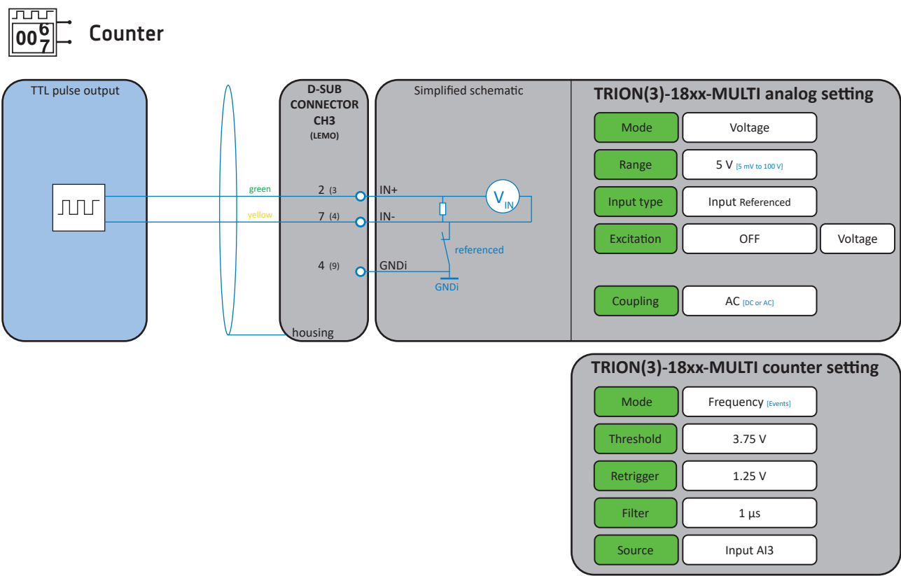
Fig. 49: Counter measurement
