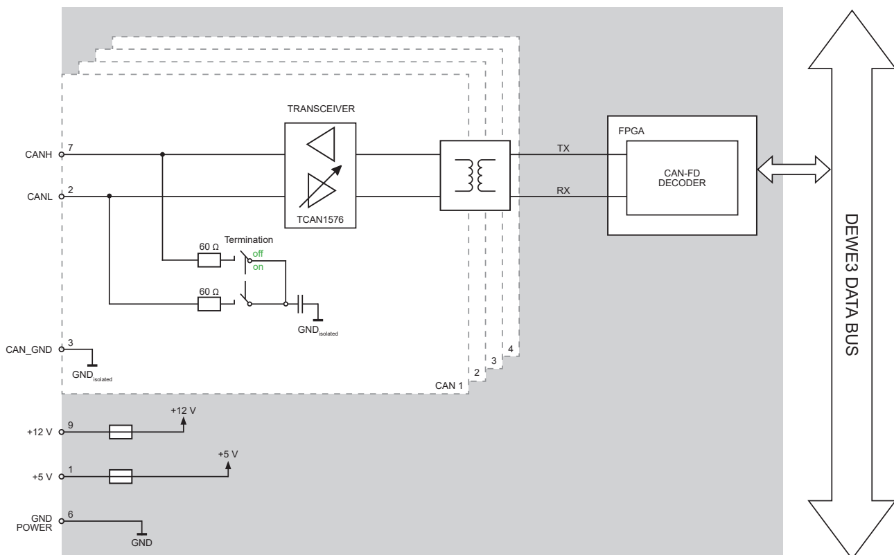
Fig. 216: Block diagram
