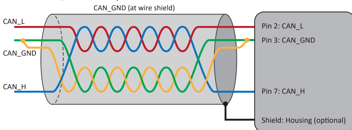
Fig. 223: Cabling for heavy industrial environment
