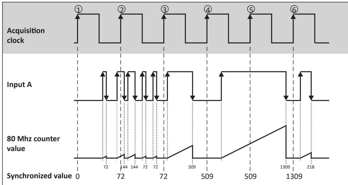
Fig. 209: Pulse width measurement
