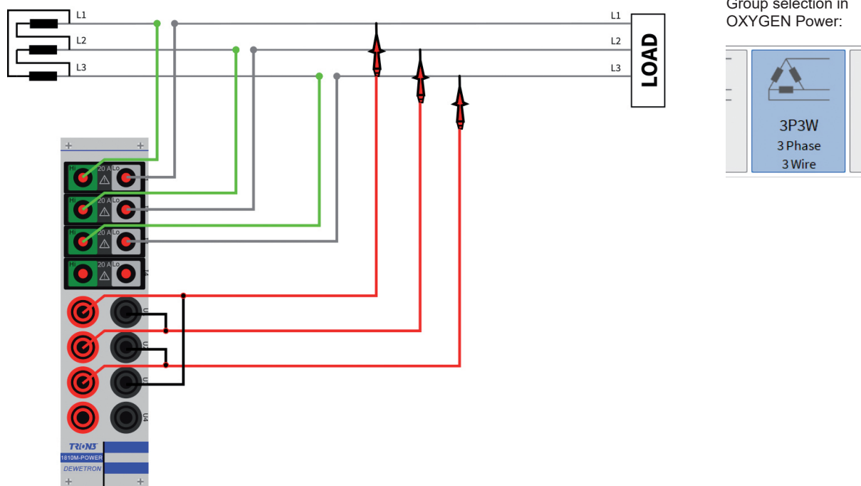
Fig. 157: Three phase (3P3W) without neutral line
