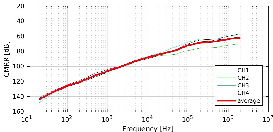
Fig. 241: CMRR over frequency response of a TRION-1820-POWER-4 (V inputs) (not a directly measured FFT chart)
