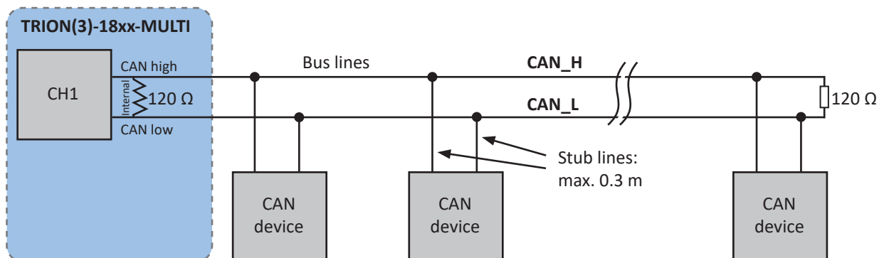
Fig. 53: CAN bus connection
