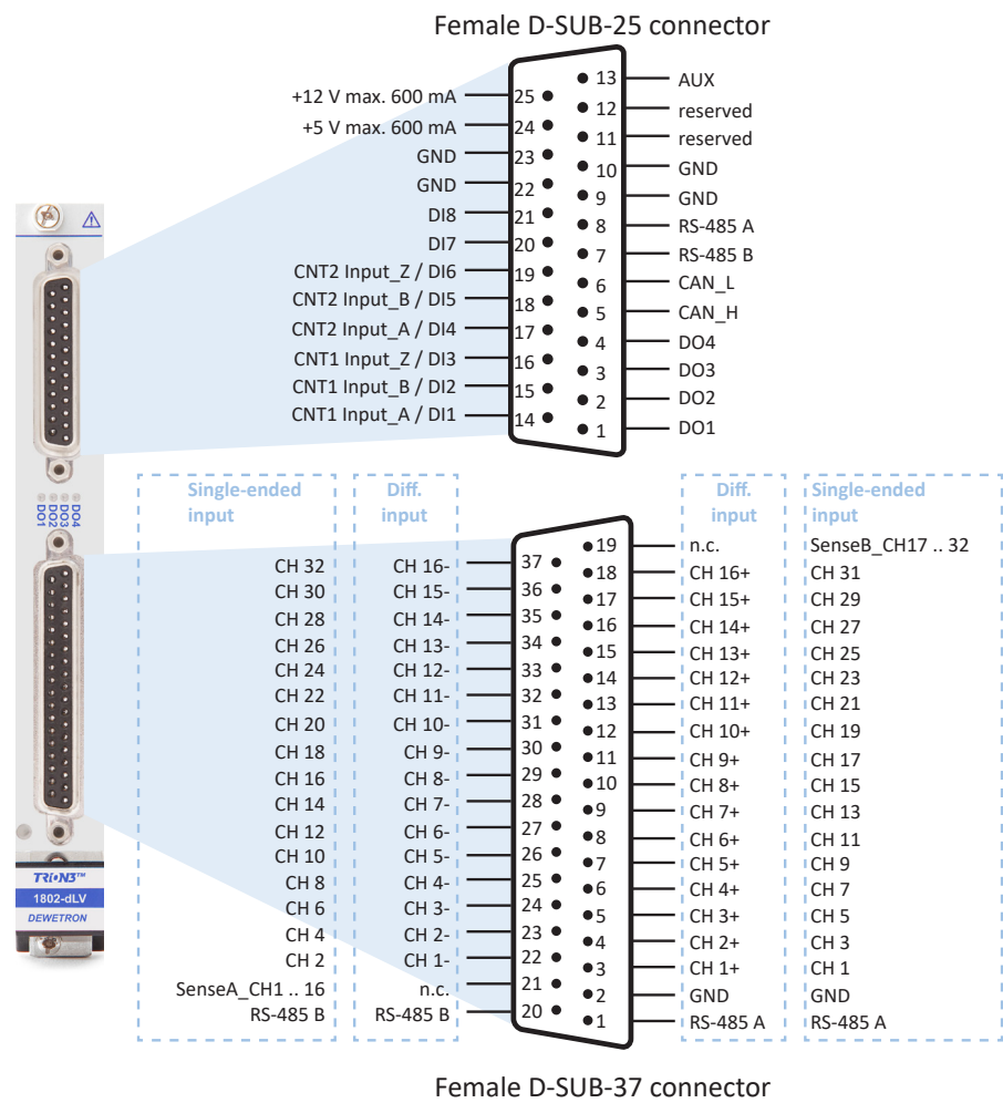
Fig. 108: Connection
