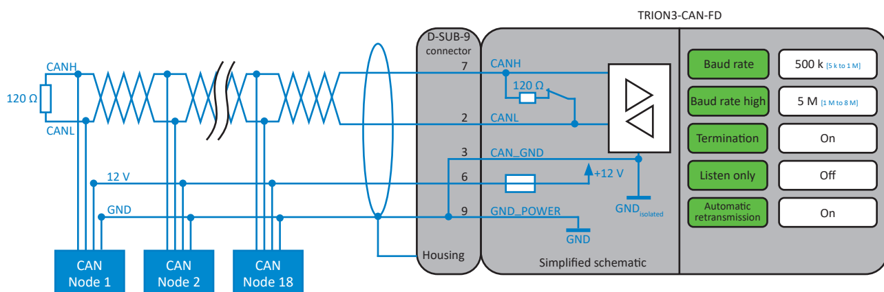
Fig. 220: Connecting sensors directly supplied by TRION3-CAN-FD
