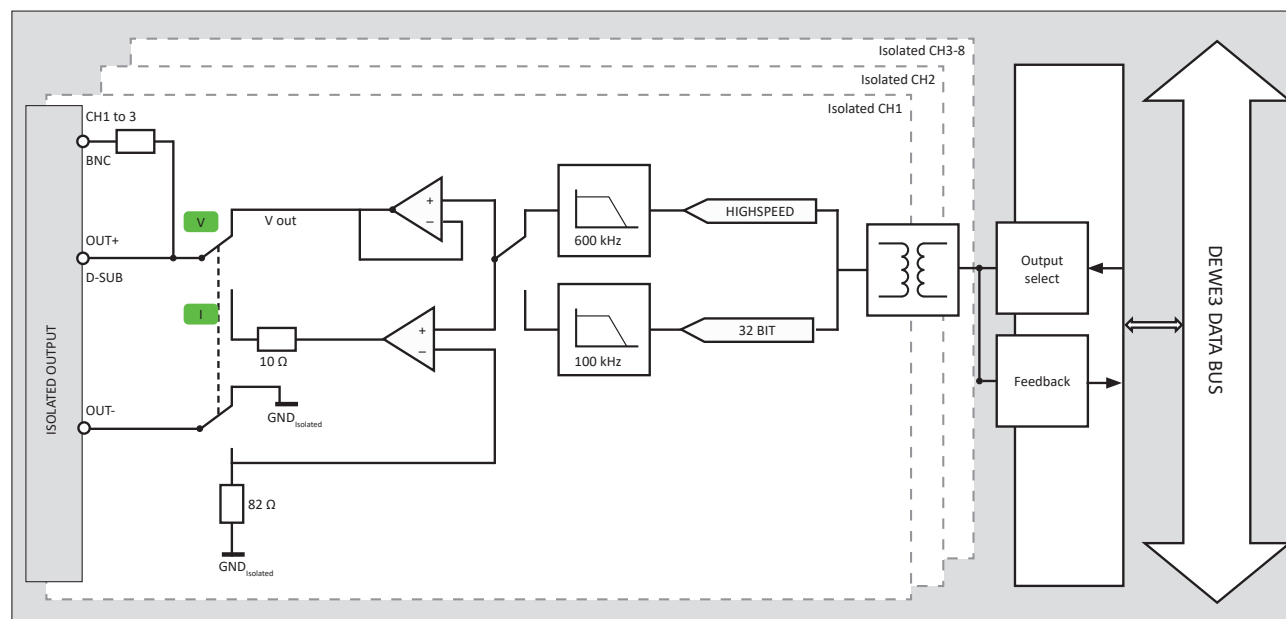
Fig. 177: Analog block diagram
