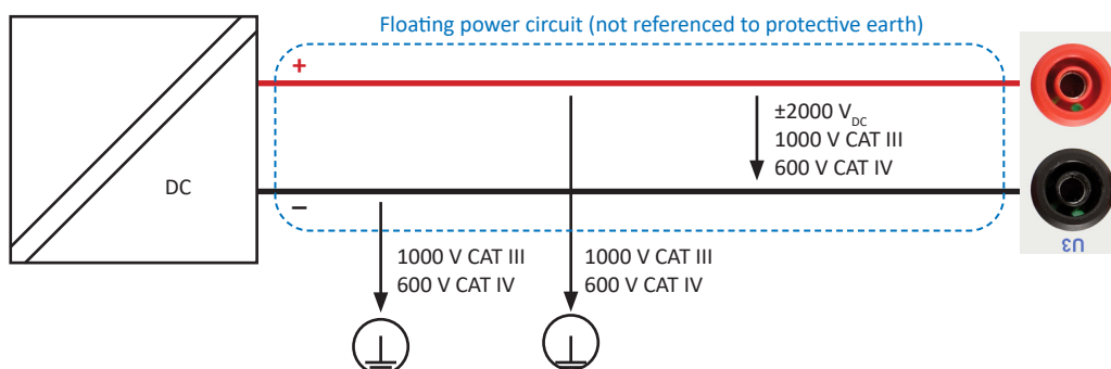
Fig. 149: Maximum input voltages
