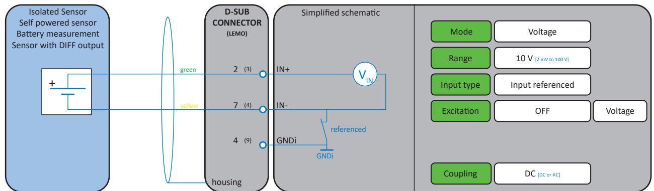
Fig. 28: Voltage measurement
