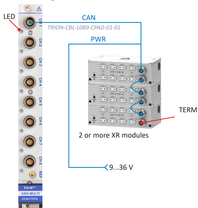
Fig. 71: Connecting XR modules to the TRION-2402-MULTI module
