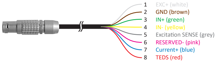
Fig. 100: TRION-CBL-L1B8-OE-05-00
