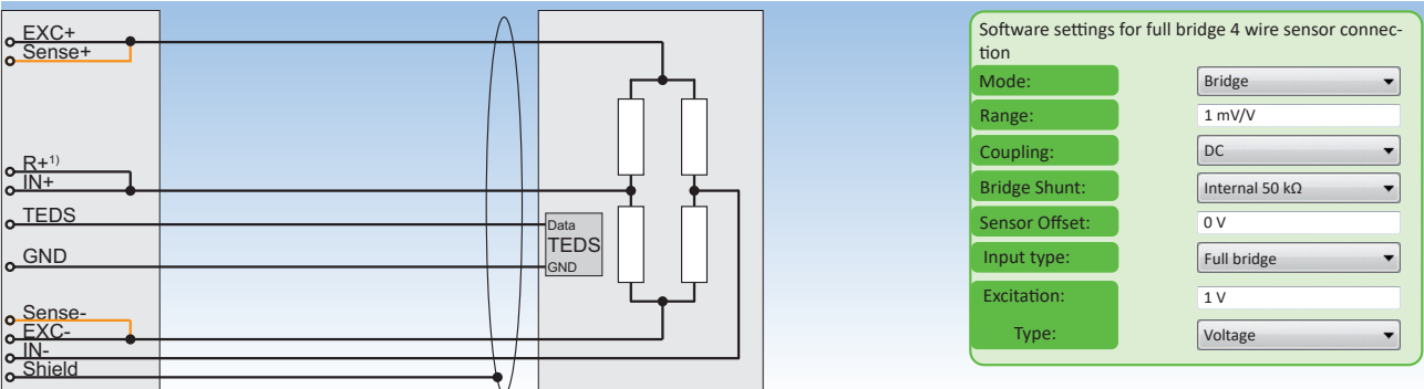
Fig. 122: Full bridge 4-wire sensor connection
