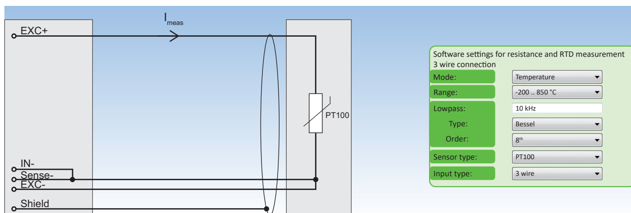
Fig. 68: Resistance and RTD measurement 3 wire connection
