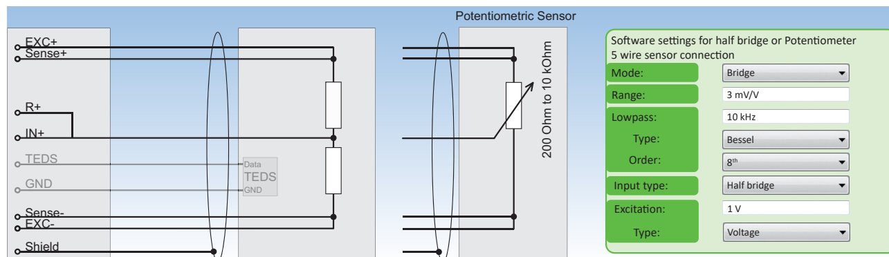
Fig. 63: Half bridge or Potentiometer 5 wire sensor connection
