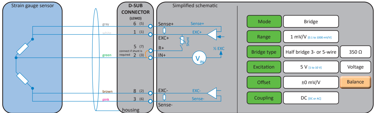
Fig. 38: Half bridge 5-wire
