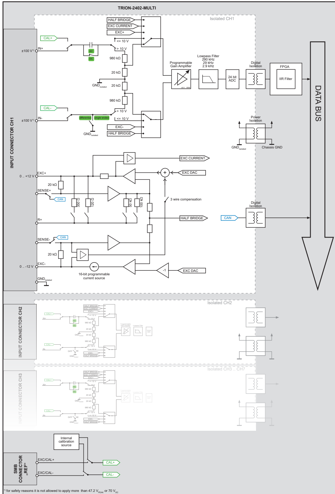
Fig. 74: Block diagram
