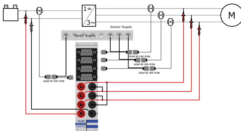
Fig. 162: Three phase and one phase (3P3W and 1P2W)
