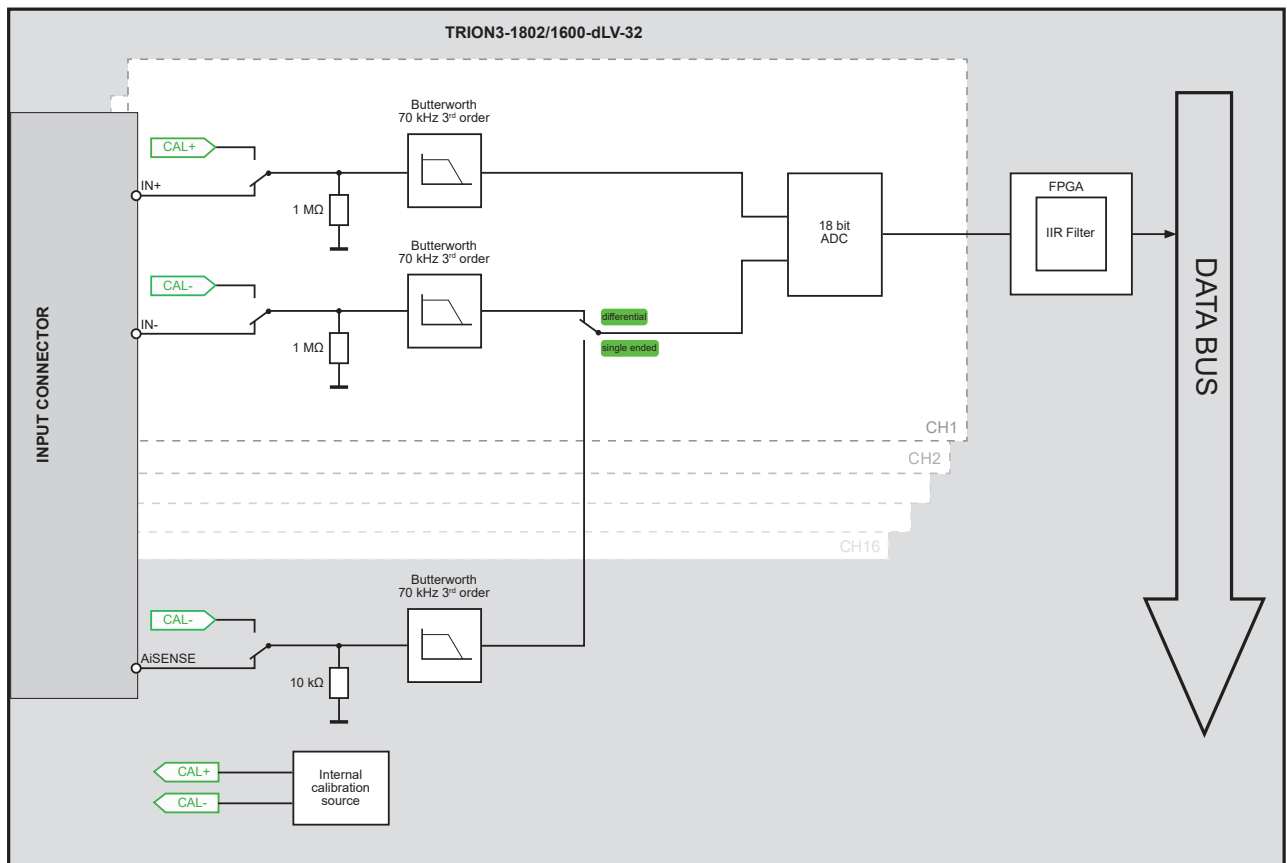
Fig. 112: Block diagram
