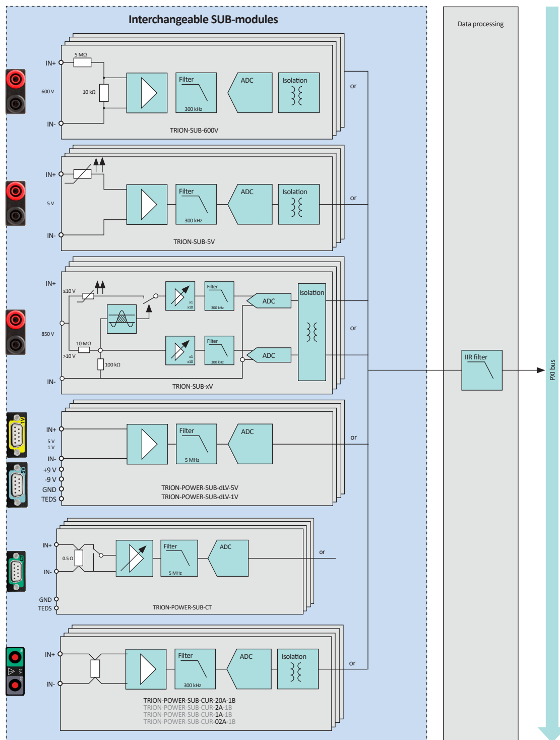
Fig. 176: Block diagram
