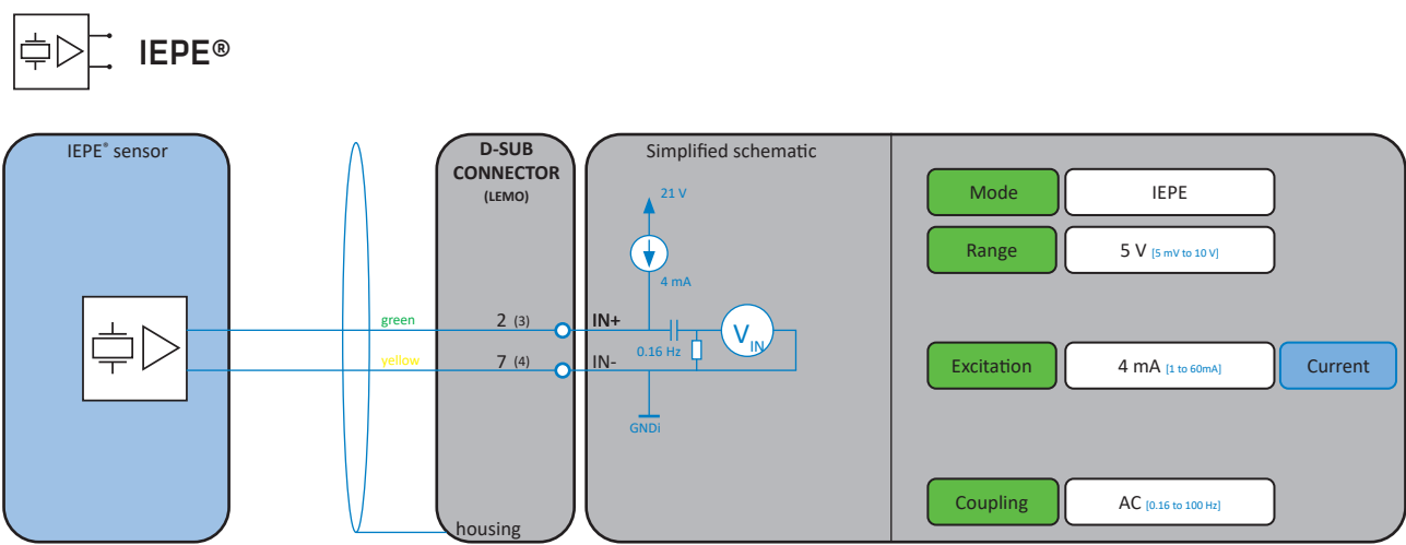
Fig. 50: IEPE® sensor
