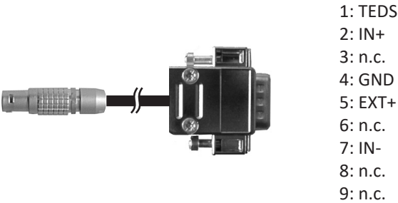
Fig. 89: TRION-CBL-L1B8-D9-0.5-01
