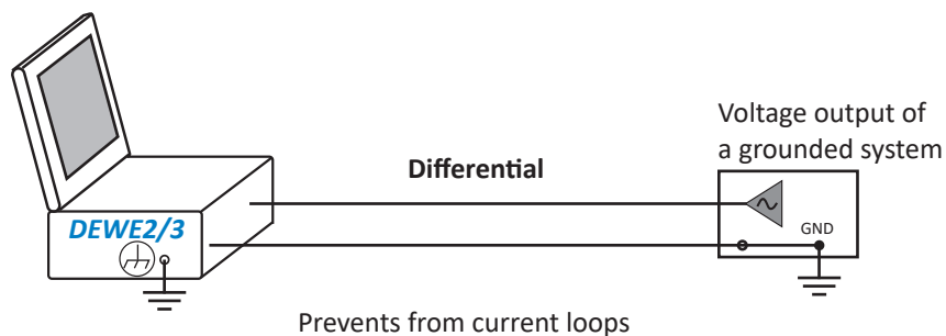
Fig. 138: Voltage output of a grounded system
