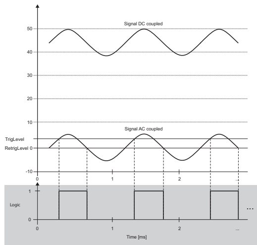
Fig. 204: Programmable trigger level
