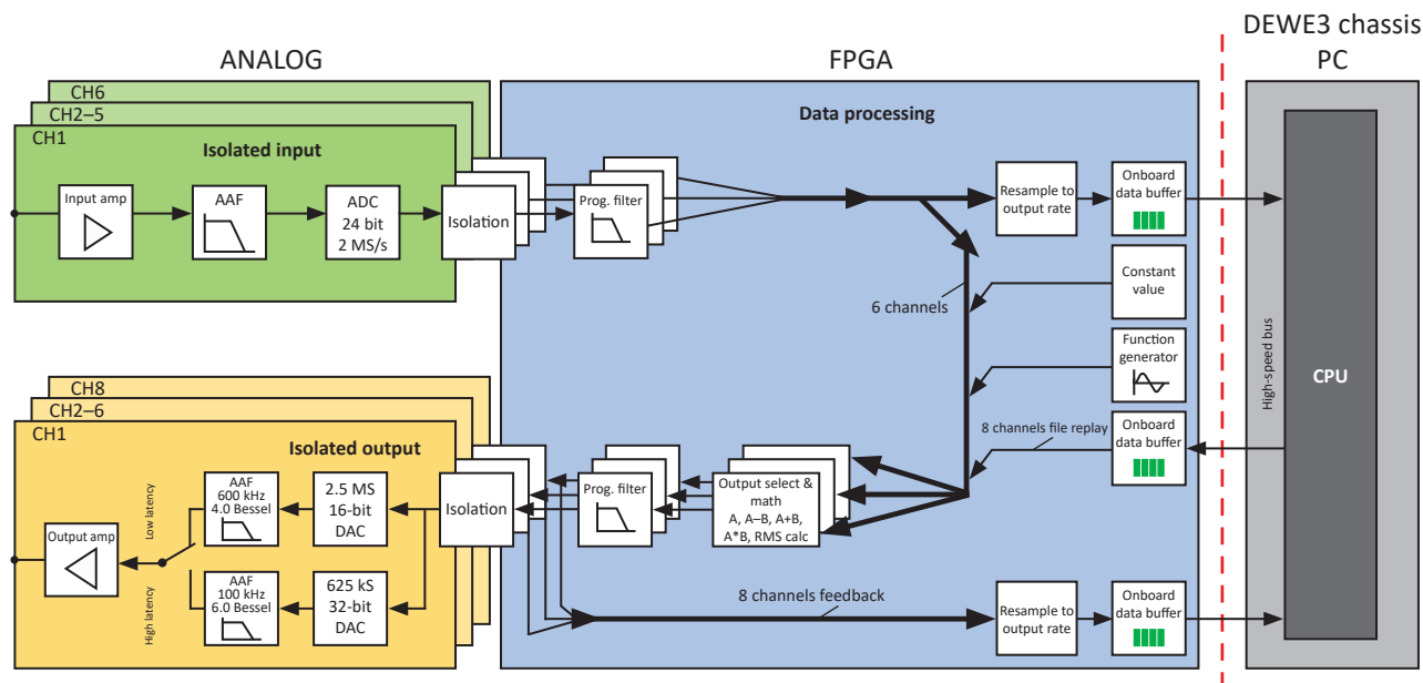
Fig. 81: Simplified signal path
