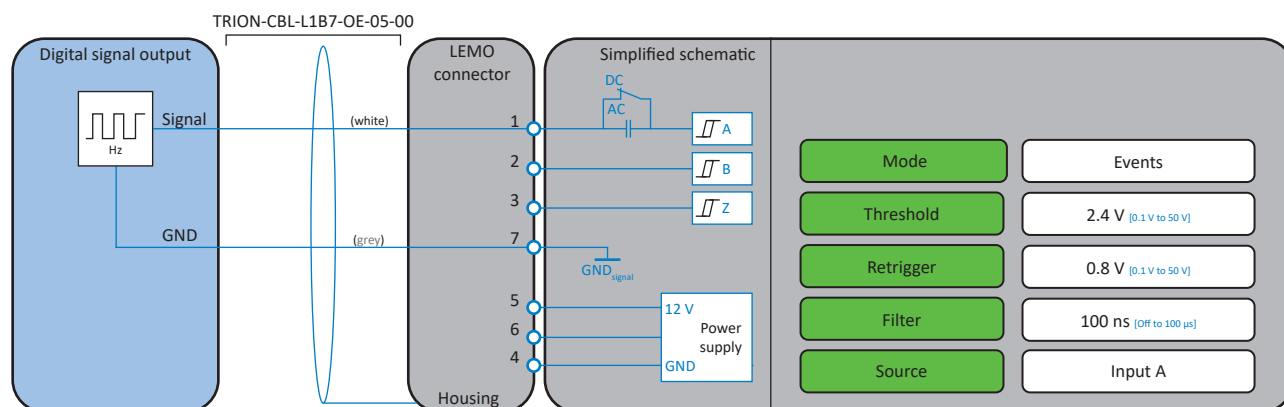
Fig. 194: Event counting (digital output)
