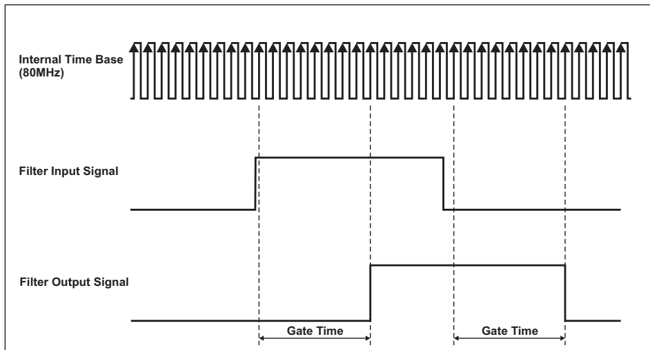
Fig. 205: Filters
