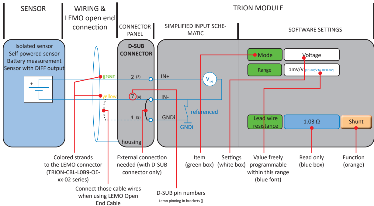
Fig. 27: Reading schematics
