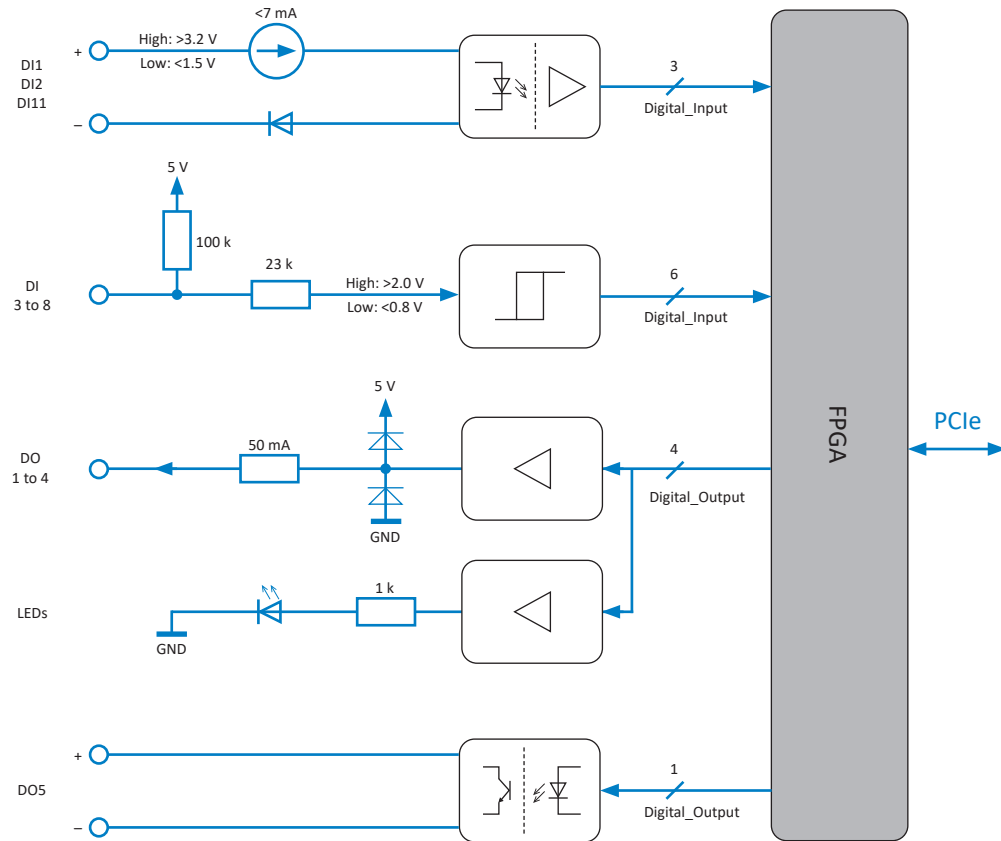
Fig. 23: Digital block diagram
