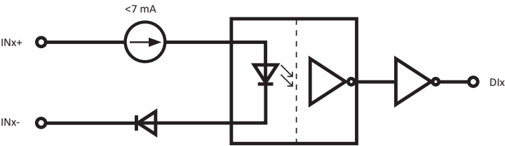
Fig. 230: Block diagram
