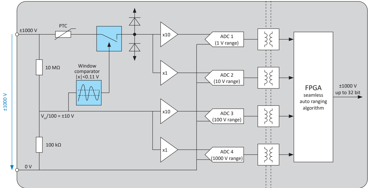
Fig. 231: Block diagram TRION-SUB-XV
