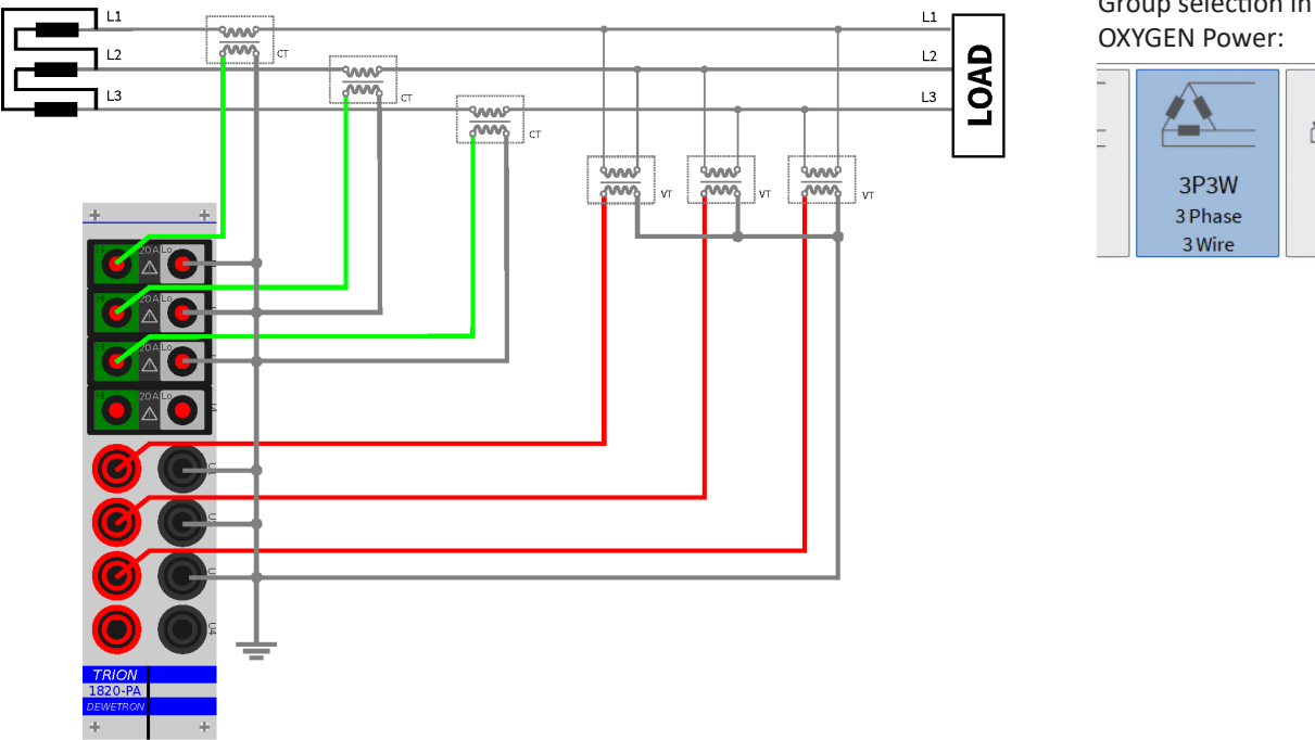
Fig. 160: Three phase (3P3W) with CT and VT
