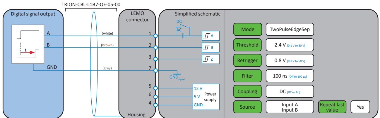
Fig. 196: Two pulse edge separation
