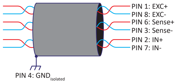
Fig. 72: Cables and shielding
