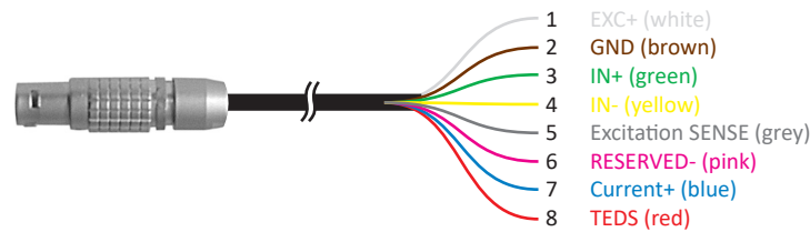
Fig. 90: TRION-CBL-L1B8-OE-05-00
